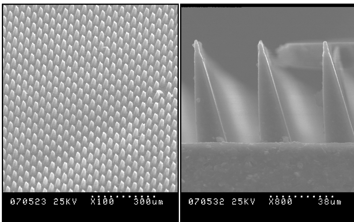
Figure 14: MicroDPS made of PDMS manufactured using a two exposure angle lithographic process to create a mold from SU-8 photoresist. Stalks shown are 20\mu\text{m} square posts, oriented vertically with an angled face. These stalks show adhesion comparable to the original DPS but require somewhat higher preloads. Stiffer materials are being used to create the microDPS that should improve durability and resistance to dirt.
