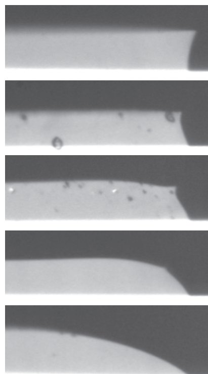
Beyond the softening point of the resist, the resist structures start to rounden. The temperature increases from top to bottom.
