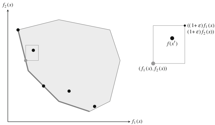
Fig. 1 Figure illustrating the concept of Pareto-optimal front (shown by the thick boundary) and approximate Pareto-optimal front (shown by solid black points) for two objectives
