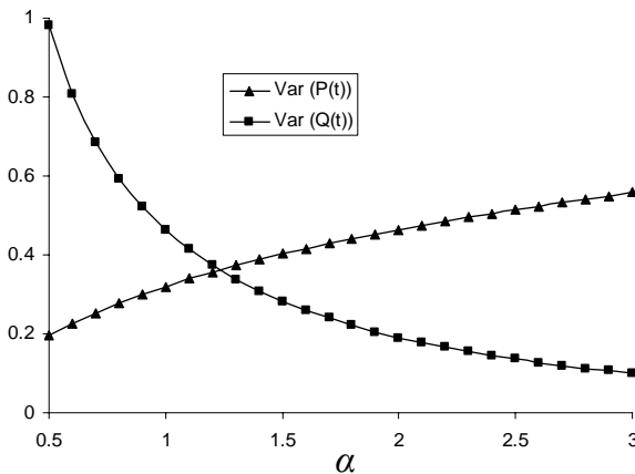
Fig. 4. Variance and P_t and Q_t as a function of \alpha for \sigma = 1
