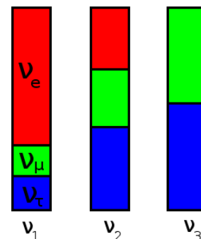
FIG. 1: The approximate flavor contents of the mass eigenstates. \nu_3 is made up nearly entirely of \nu_\mu and \nu_\tau eigenstates; the mixing with \nu_e is too small to be shown in this figure
