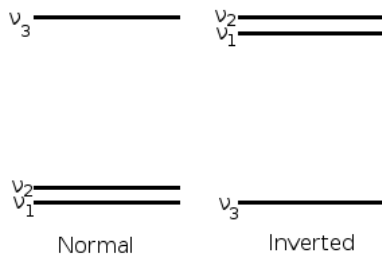
FIG. 2: The normal and inverted relative neutrino mass spectra
