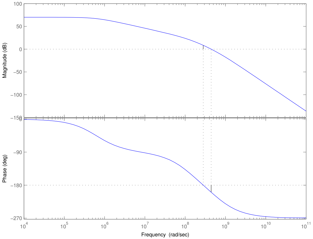
Bode Diagram Gm = -8.37 dB (at 2.81e+008 rad/sec) , Pm = -19.3 deg (at 4.42e+008 rad/sec)
