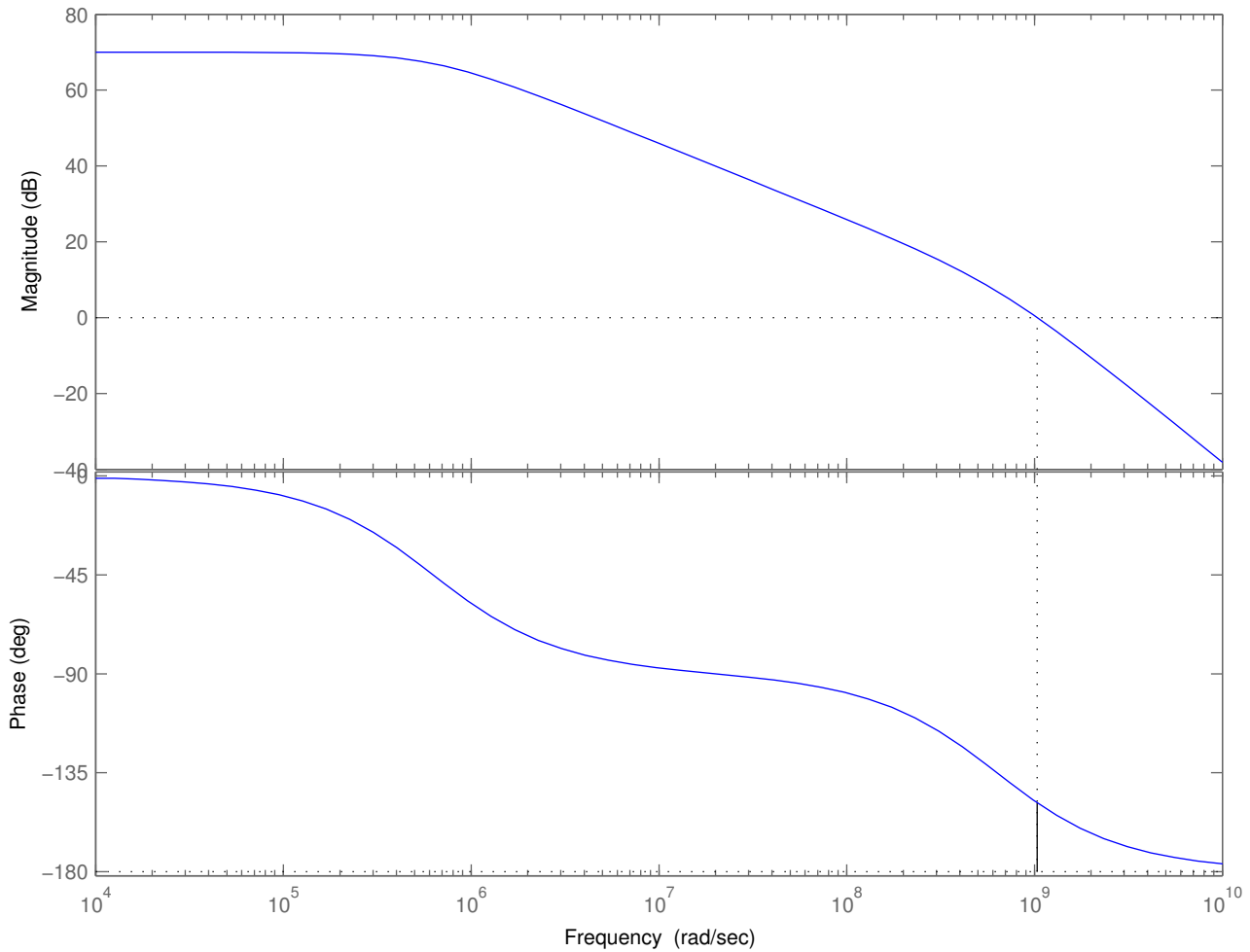
Bode Diagram Gm = Inf dB (at Inf rad/sec) , Pm = 31.4 deg (at 1.03e+009 rad/sec)
