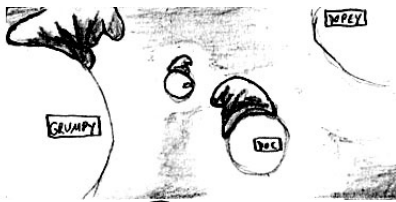
WHITE DWARF
