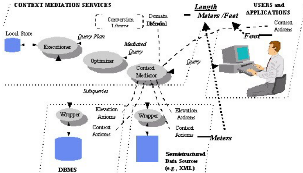
Figure 1. The Architecture of The Context interchange System
