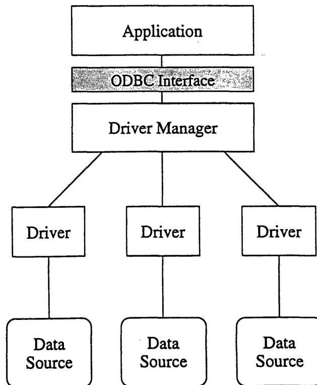
Figure 2.2-1: ODBC architecture
