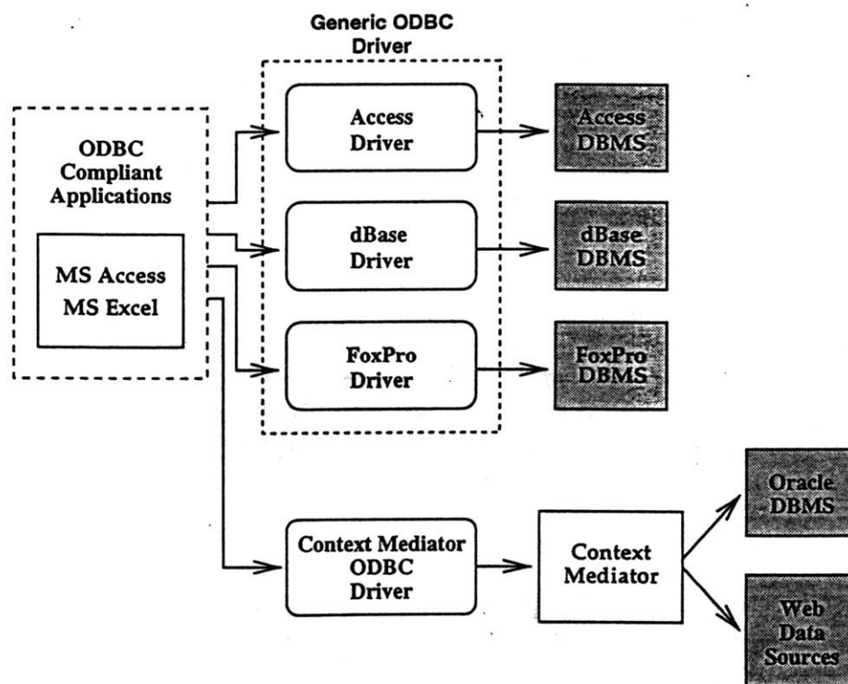
Figure 3.1-1: Overview of the ODBC Framework
