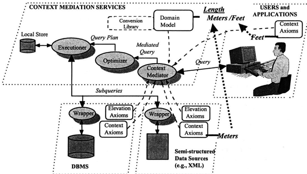
Figure 4. The Architecture of the Context Interchange System
