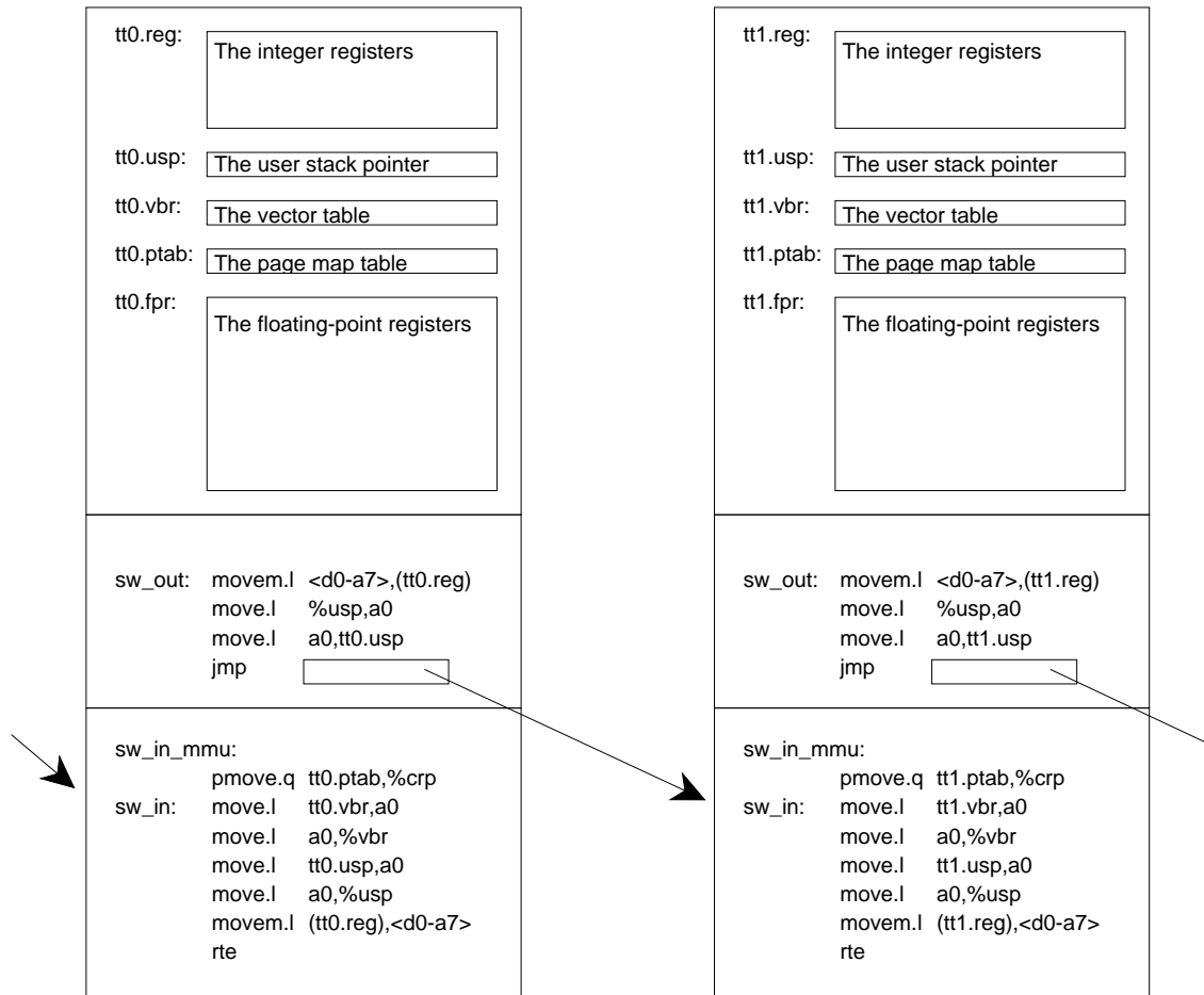
Figure 3.4: Thread Context
