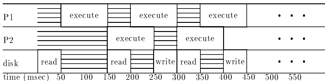
Figure 6.8: Two Processors, Static Scheduling
