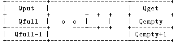
Figure 4.1: Queue Quaject
