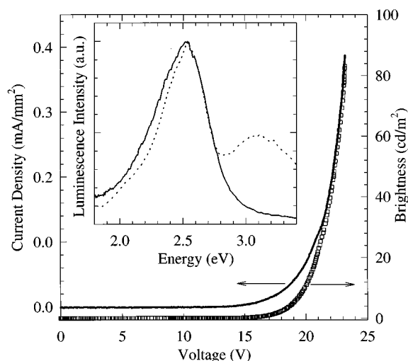
FIG. 5. Current–voltage (—) and brightness–voltage (□) characteristics of a typical bilayer light-emitting device. Inset: PL (···) and EL (—) of a bilayer light-emitting device.
