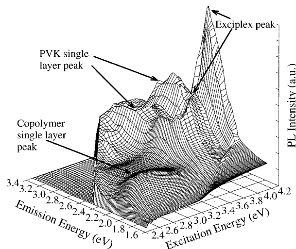
FIG. 3. PL of a bilayer of PVK and PPyVP(COOC 12 H 25 ) 2 V as a function of both emission energy and excitation energy. The 3D plot shows three prominent features: a peak due to the PVK (excitation energy from 3.6 to 4.2 eV, emission energy 2.8 to 3.4 eV), a peak due to the copolymer (excitation energy from 2.4 to 3.0 eV, emission energy 1.8 to 2.2 eV), and the exciplex peak (excitation energy from 3.6 to 4.2 eV, emission energy 2.2 to 2.8 eV).
