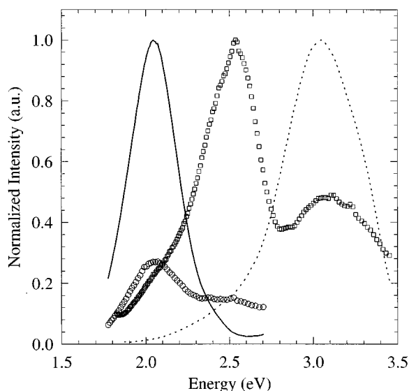
FIG. 2. PL of PPyVP(COOC 12 H 25 ) 2 V at 2.8 eV excitation energy (—), a bilayer of PVK and PPyVP(COOC 12 H 25 ) 2 V at 3.6 eV excitation energy (□) and 2.8 eV excitation energy (○), and PVK at 3.6 eV excitation energy (···), all on quartz substrates.
