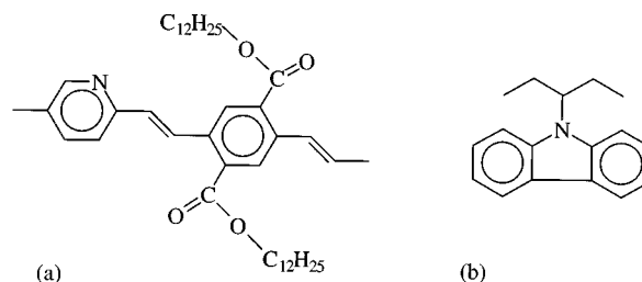
FIG. 1. Molecular repeat unit of (a) PPyVP(COOC 12 H 25 ) 2 V and (b) PVK.
