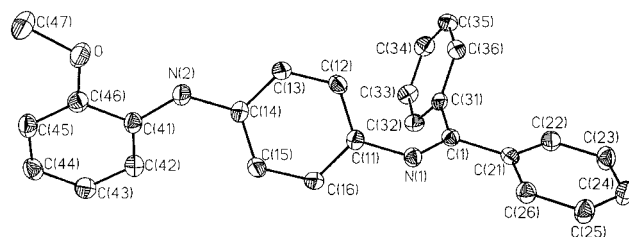
Figure 1. Single-crystal X-ray structure of protected oligomer 3 . Selected bond lengths and angles: O–C(46) 1.373(3), O–C(47) 1.428(3), N(2)–C(41) 1.389(3), N(2)–C(14) 1.402(3), N(1)–C(11) 1.420(3), N(1)–C(1) 1.281(3) Å; C(46)–O–C(47) 117.3(2), O–C(46)–C(45) 125.5(3), C(14)–N(2)–C(41) 129.2(2), C(1)–N(1)–C(11) 124.0(2)°.
