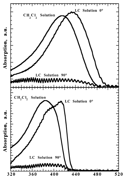
Figure 1. Absorption spectra taken at rt of 1d (top) and 2a bottom in \text{CH}_2\text{Cl}_2 and 6CHBT. The red-shift in the liquid crystal solution is clearly apparent, and the alignment is apparent from the ratio of the spectra taken at 0^\circ and 90^\circ to the nematic director. The periodic signal at 90^\circ is due to interference effects from the rubbed polyimide coatings.
