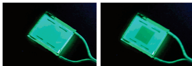
Figure 2. Fluorescent image of a test cell containing 1d in 6CHBT. At the left a test cell is shown with no applied voltage, and the nematic director and polymer are aligned with the short axis of the cell. At the right, 9 V is applied between ITO pads on the top and bottom of the test cell that realigns the liquid crystal and polymer normal to the glass slides.
