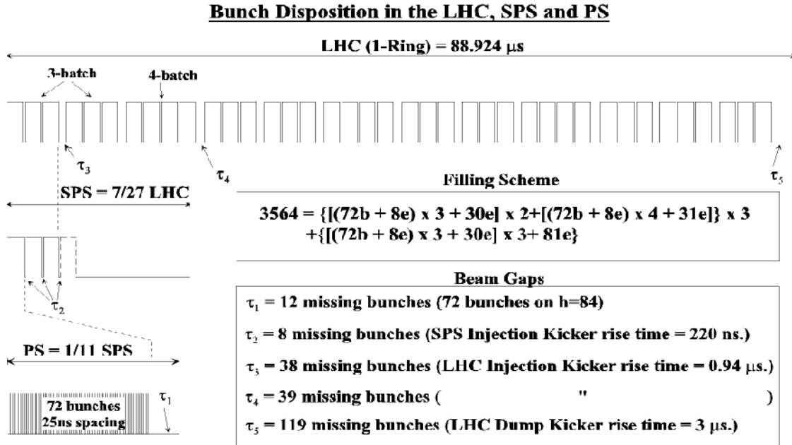
Figure 12.2: Proton bunches in the PS, SPS and one LHC ring. Note the partial filling of the SPS (3/11 or 4/11) and the voids due to kicker rise-time. One LHC ring is filled in \sim 3 min.
