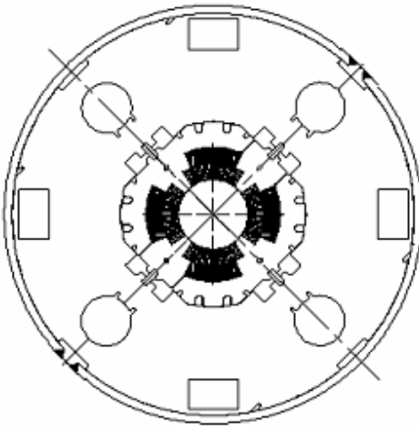
Figure 3.18: Cross-section of the MQXB low- \beta quadrupole (left) and Q2 quadrupole on test in FNAL (right).
