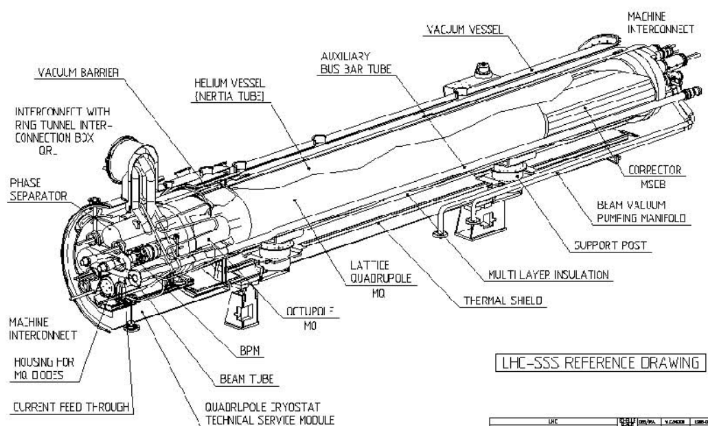
Figure 3.6: Short straight section with jumper.
