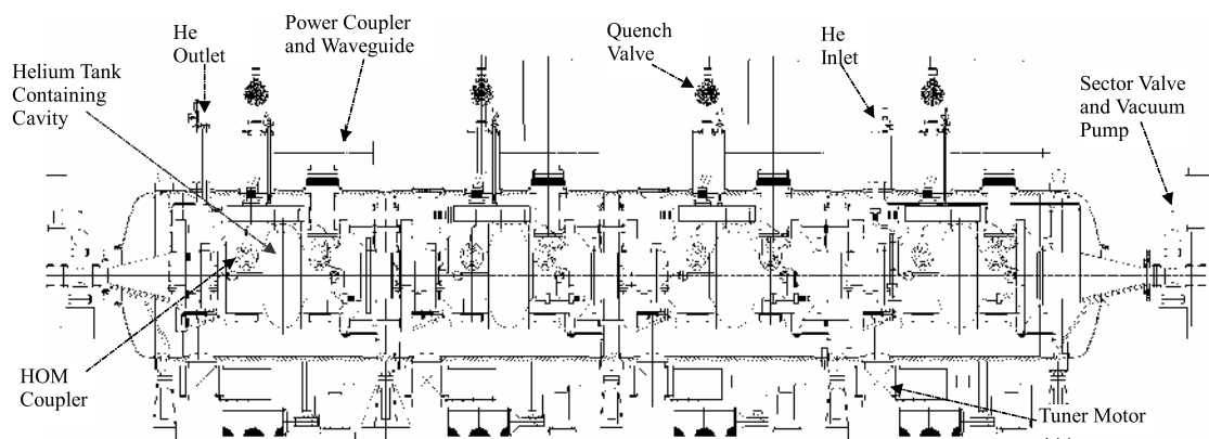
Figure 4.1: Four-cavity cryomodule.
