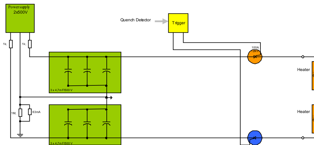
Figure 6.7: Quench heater power supply functional diagram.
