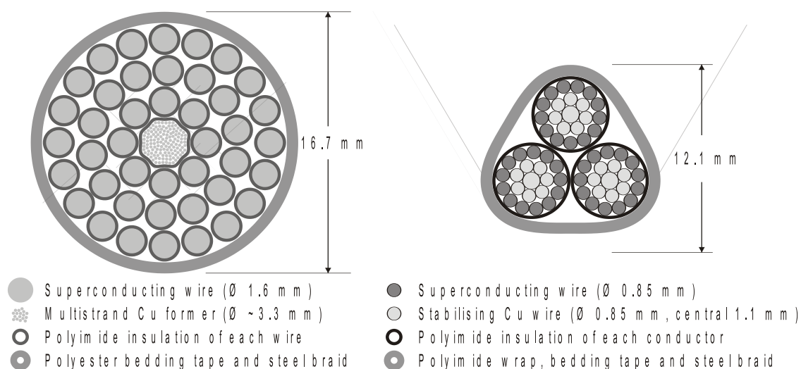
Figure 6.6: Cross sections of the 42 \times 600 A cable (left) and the 3 \times 6 kA cable (right).
