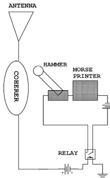
Figure 2: Receiving apparatus using a coherer
