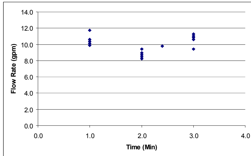
Figure 48: Flow-Rates From Gravity-Fed Tank in Cambridge
