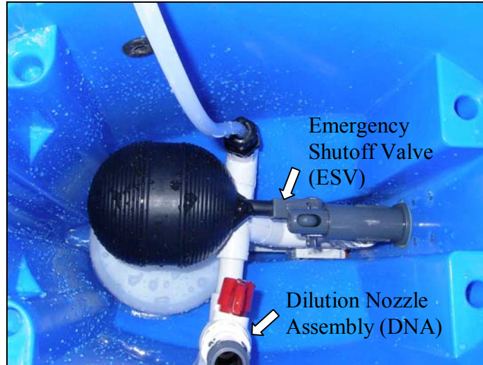
Figure 39: Emergency Shutoff Valve (ESV) & Dilution Nozzle Assembly (DNA) Modifications Tested in Cambridge
