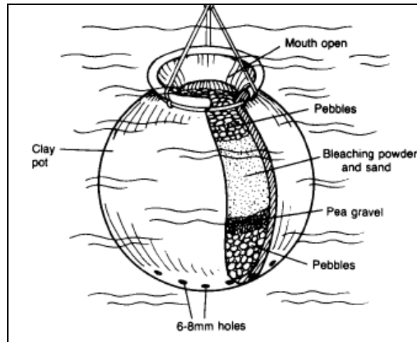
Figure 9: Design of a Pot Chlorinator (Water for the World 2007)
