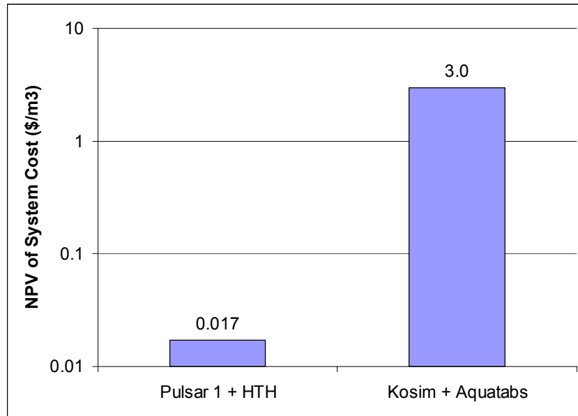
Figure 52: Net Present Value (NPV) Comparison of Pulsar 1 + HTH versus Kosim + Aquatabs, Normalized to Treatment Cost per Volume
