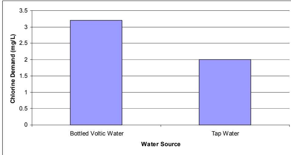
Figure 34: Chlorine Demand Comparison of Tap and Local Bottled Water in Tamale
