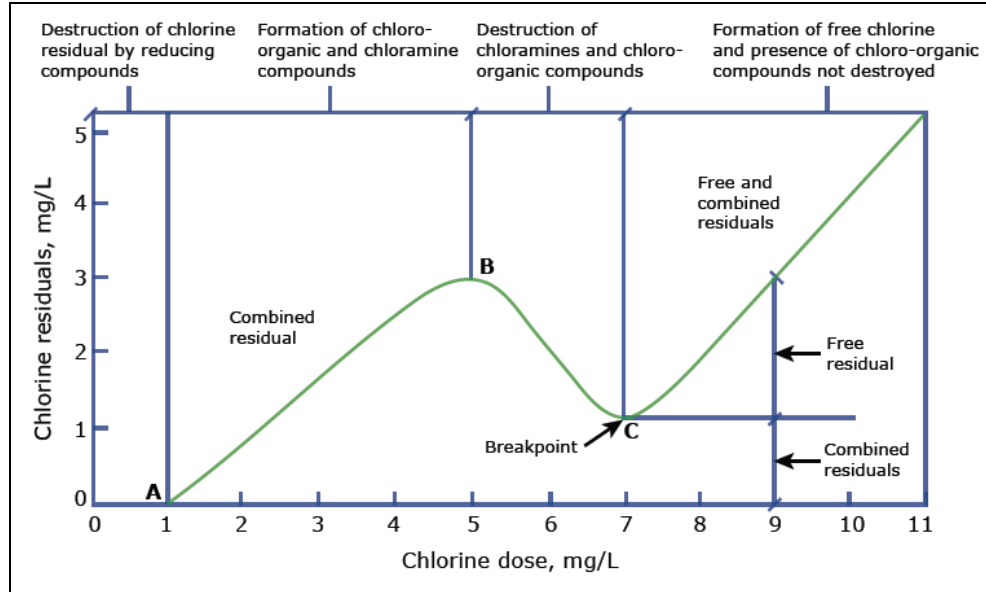
Figure 18: Typical Break-point Chlorination Curve (Metcalf & Eddy 2003)
