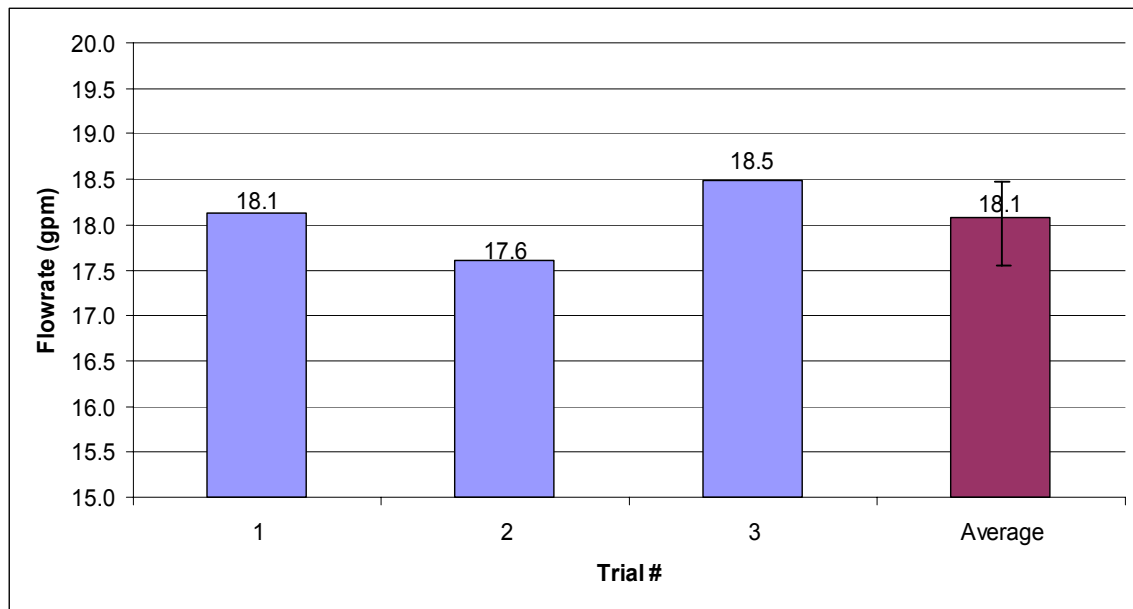
Figure 40: Flow-Rates From Gravity-Fed Tank in Ghana
