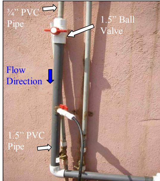
Figure 32: PVC Connections from Elevated Tank to Storage Tank in Ghana
