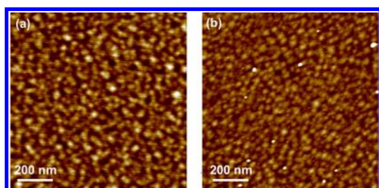
Figure 2. LSC morphology on (a) STO and (b) LAO showed smooth surfaces with RMS roughnesses of 0.64 \pm 0.06 and 0.56 \pm 0.05 nm, respectively, imaged by atomic force microscopy.
