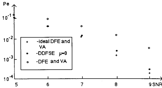
Fig. 11. Example 5. Rate 2/3, 8-PSK system followed by a channel with response 1/(1 - 0.5D) . \text{SNR} = A^2/N_0 .
