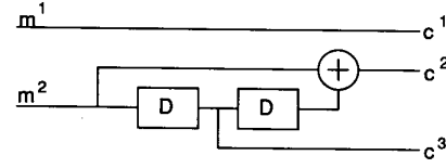
Fig. 8. The (3,2) BCC.
