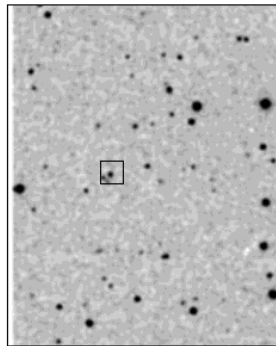
2MASS J
