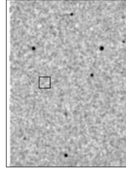
2MASS K s
