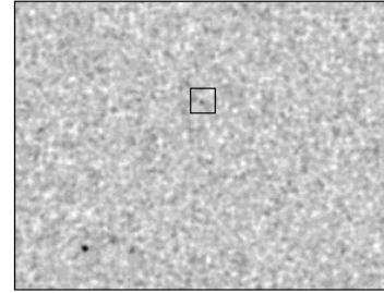
2MASS K s
