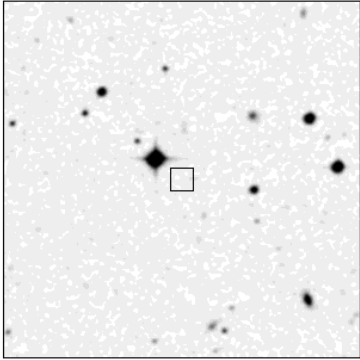
SERC R
