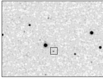
2MASS J
