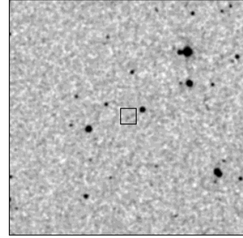
2MASS K s
