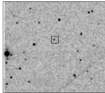
2MASS J
