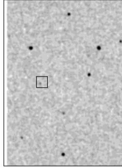
2MASS J
