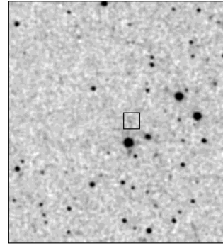
2MASS K s
