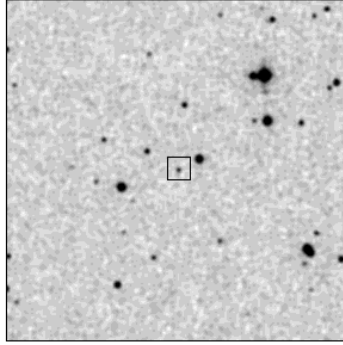
2MASS J
