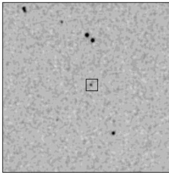
2MASS J
