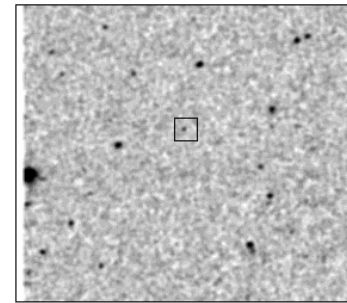
2MASS K s
