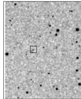
2MASS K s
