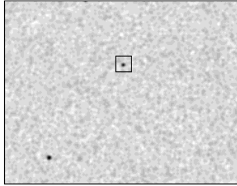
2MASS J
