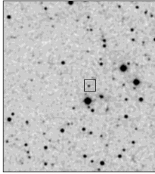
2MASS J
