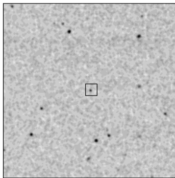
2MASS J
