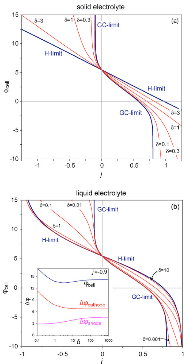
Fig. 3. Cell voltage vs. current for a galvanic cell with fixed (a) and mobile (b) countercharge, operating in all three modes identified in Fig. 1 in the thin-diffuse layer (zero- \varepsilon ) limit based on Eqs. (23)–(36) ( j_{0,A} = 0.8 , j_{0,C} = 0.1 , k_{R,A} = 1 , k_{R,C} = 30 ). Reaction-limited current is obtained in the GC-limit when j \rightarrow j_{0,A} or j \rightarrow -j_{0,C} , while in the H-limit the current is diffusion-limited when j \rightarrow \pm 1 , but only for mobile countercharge. Insert in (b) shows non-monotonic dependence of \phi_{\text{cell}} on \delta .
