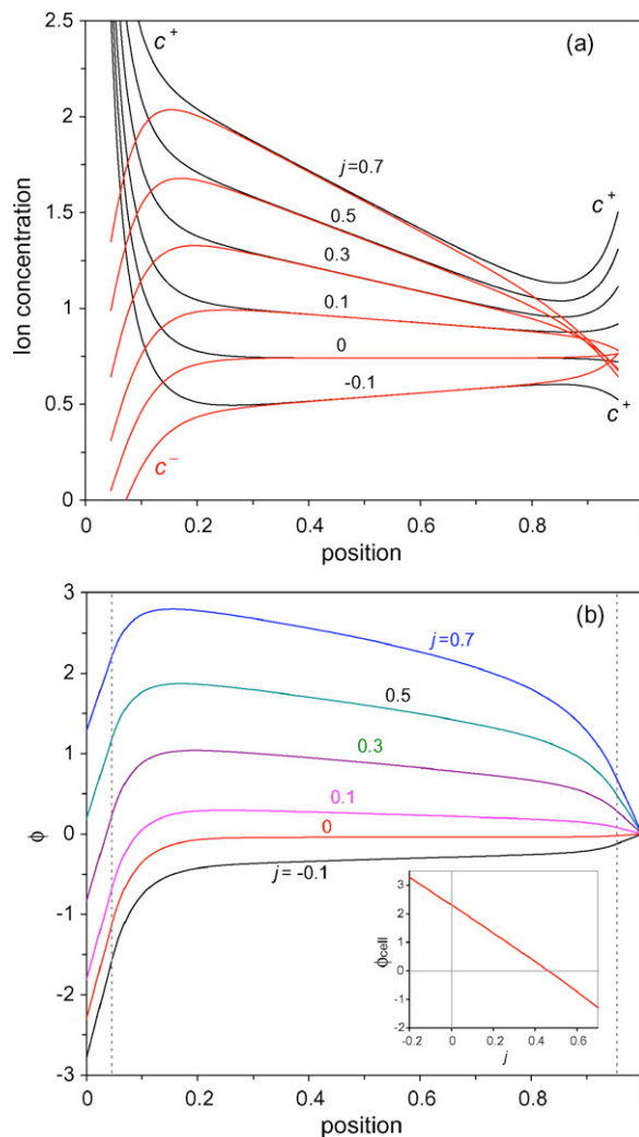
Fig. 9. Ion concentration and potential profiles in a liquid galvanic cell with reactive cations and all ions mobile (parameter settings as in Fig. 8 except for current j ). Concentrations are shifted vertically in a). Dashed vertical lines in b) denote the Stern planes. The insert picture presents the cell voltage as function of current.
