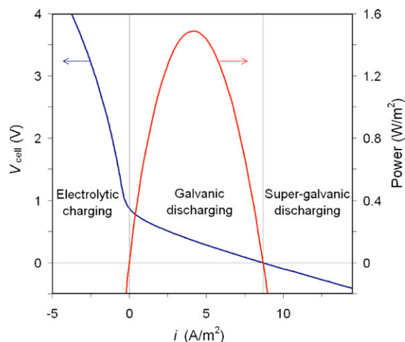
Fig. 1. Regimes of operation of a galvanic cell with imposed current. The calculations are based on a proton conducting fuel cell (see parameter settings of Fig. 3).
