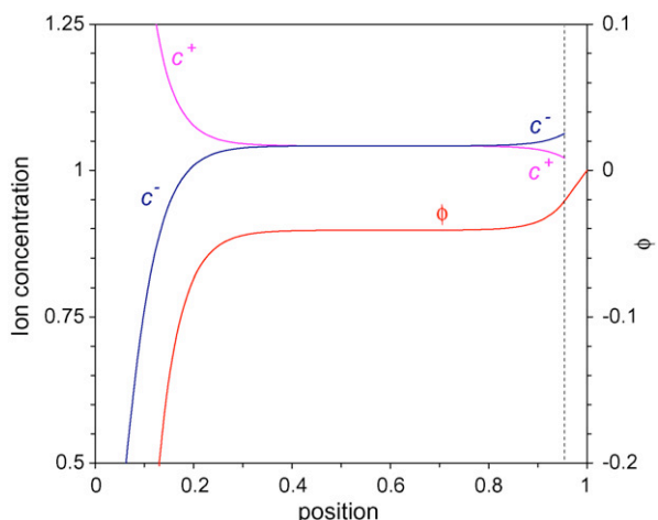
Fig. 8. Equilibrium ion concentration and potential profiles in a liquid galvanic cell with reactive cations and all ions mobile (open-circuit condition, thus current j=0 , \delta=1 , j_{O,A}=10 , j_{O,C}=1 , k_{R,A}=k_{R,C}=1 , \varepsilon=0.05 ). Anode located left, cathode right.
