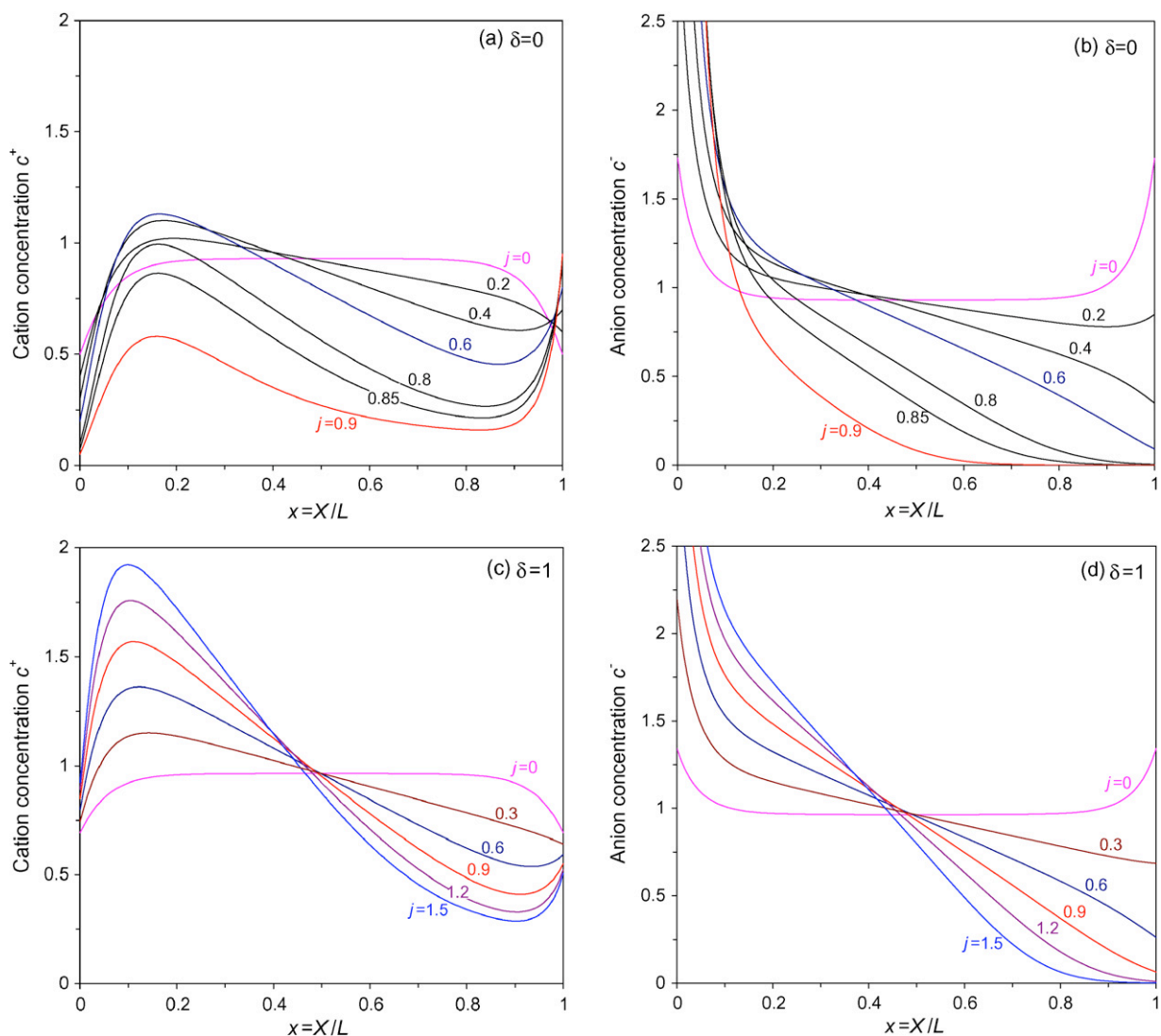
Fig. 7. Ion concentration profiles in a liquid electrolytic cell with reactive cations and all ions mobile, at various values of the current j and for \delta = \lambda_s/\lambda_D either zero or unity (on both electrodes: j_{O,i} = 1 , k_{R,i} = 2 , \varepsilon = \lambda_D/L = 0.05 ) as function of x = X/L . Anode located left, cathode right.
