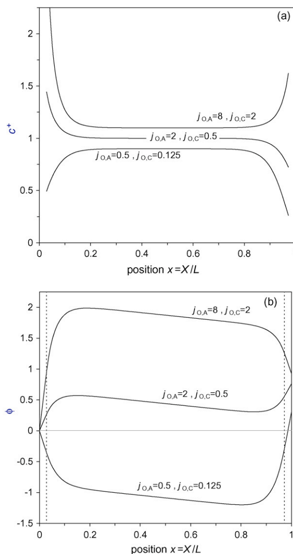
Fig. 6. Proton concentration ( c^* ) and electrostatic potential ( \phi ) profiles for a galvanic cell with fixed countercharge (dimensionless current j = 0.1 , \varepsilon = 0.03 , k_{R,A} = k_{R,C} = 1 ). In all cases the open cell voltage is the same, namely \phi_0 = \ln(j_{0,A}/j_{0,C}) \sim 1.39 .
