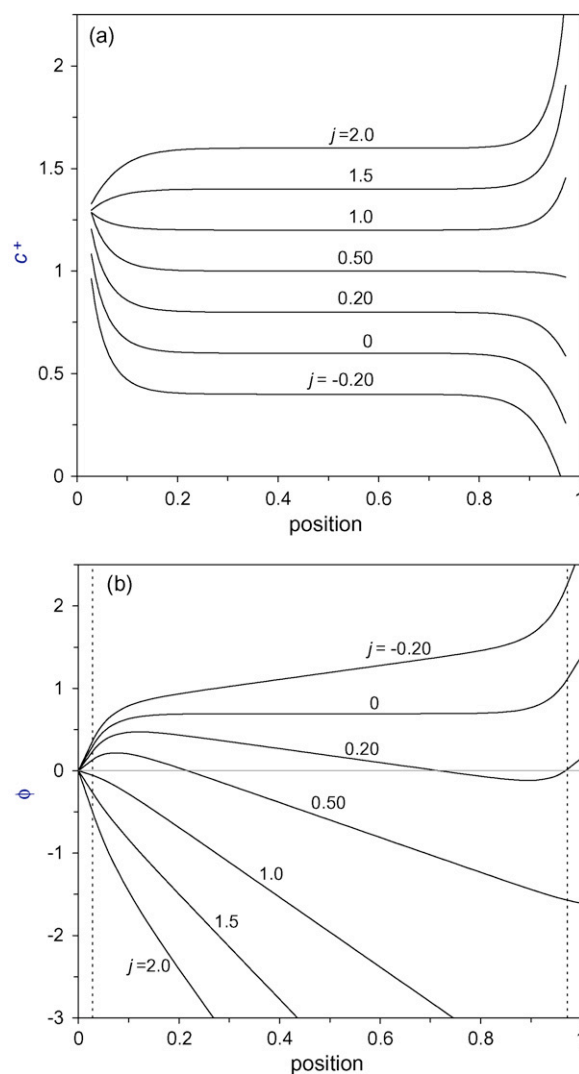
Fig. 5. Proton concentration ( c^+ ) and electrostatic potential ( \phi ) profiles for a fuel cell with fixed countercharge operated at various values of the dimensionless current j . The anode is located left and the cathode right. For currents 0 \leq j \leq 0.20 the cell functions as a galvanic cell while outside this range a current must be imposed on the cell. Dashed lines in (b) denote the Stern plane. In (a) the profiles are shifted up- and downward for clarity; in the bulk the dimensionless concentration is \sim 1 for all conditions.
