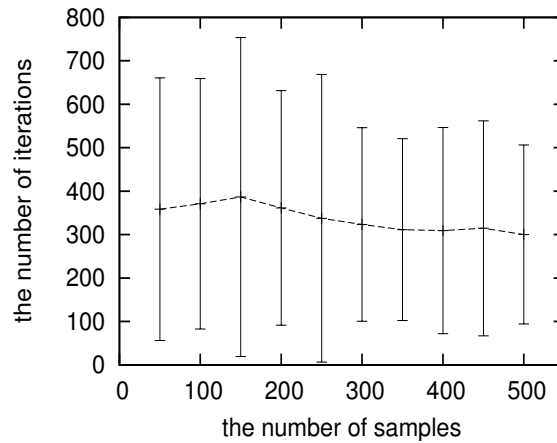
Figure 3: The number of iterations of PE with 10 classes. Each error bar represents the standard deviation of 1000 results with different initial conditions.
