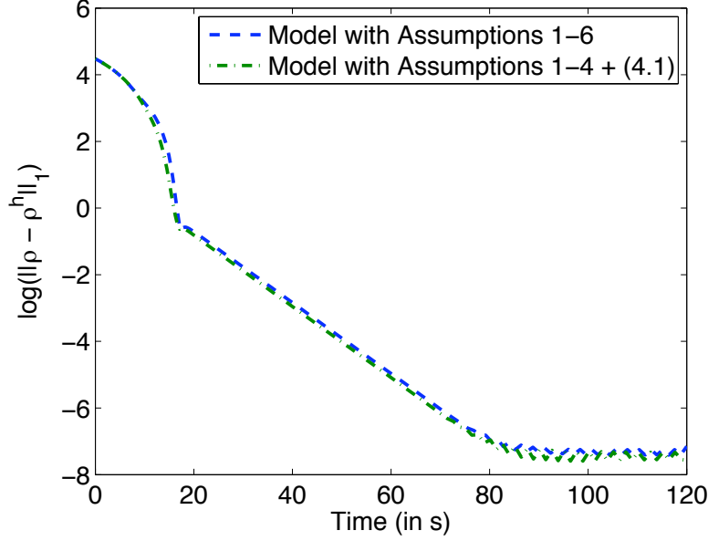
FIG. 4.2. Log-linear plot for comparison of the evolution of \|\rho(t) - \rho^h\|_1 for the local decision function of Example 3 versus the local decision function of (4.1).
