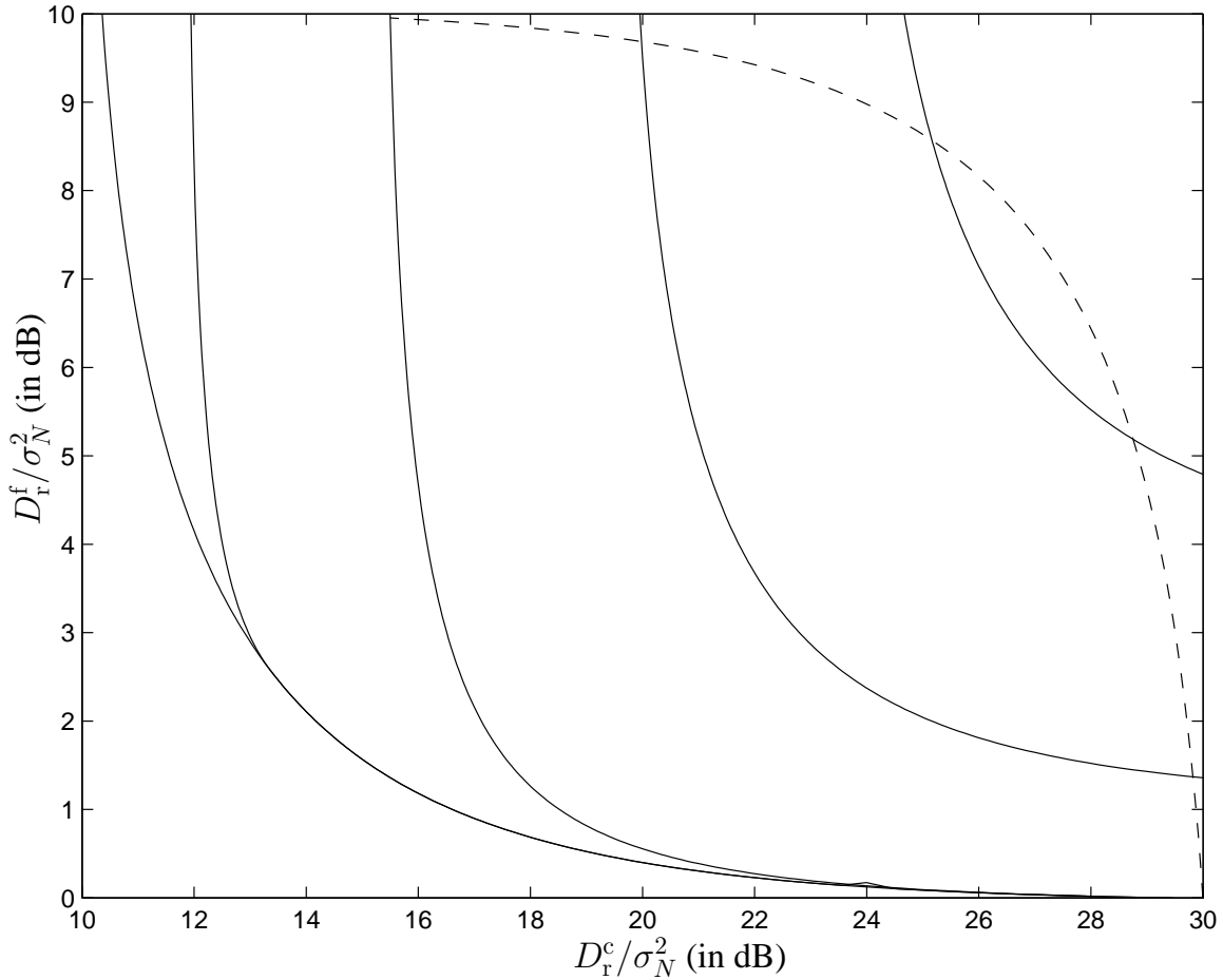
Fig. 10. Achievable fine and coarse quality reconstruction distortion pairs (D_r^f, D_r^c) in a layered authentication system for the Gaussian-quadratic case with \sigma_S^2/\sigma_N^2 = 30 dB, \sigma_V^2/\sigma_N^2 = 10 dB, and \sigma_N^2 = 1 . From left to right, the curves are the boundaries of achievable distortion regions corresponding to encoding distortions of D_e/\sigma_N^2 = 10, 5, 0, -5, -10 dB. The dashed curve corresponds to time-sharing between two operating points on the D_e/\sigma_N^2 = 0 dB curve.
