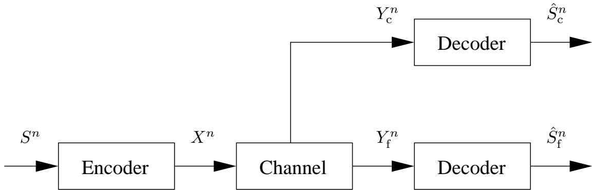
Fig. 8. Two-layer authentication system operation when the reference channel is in effect. From the outputs Y_f and Y_c of the degraded broadcast reference channel, corresponding to mild and harsh editing, the respective fine and coarse authentic reconstructions \hat{S}_f^n and \hat{S}_c^n are produced. The common encoding obtained from the source S^n is X^n .
