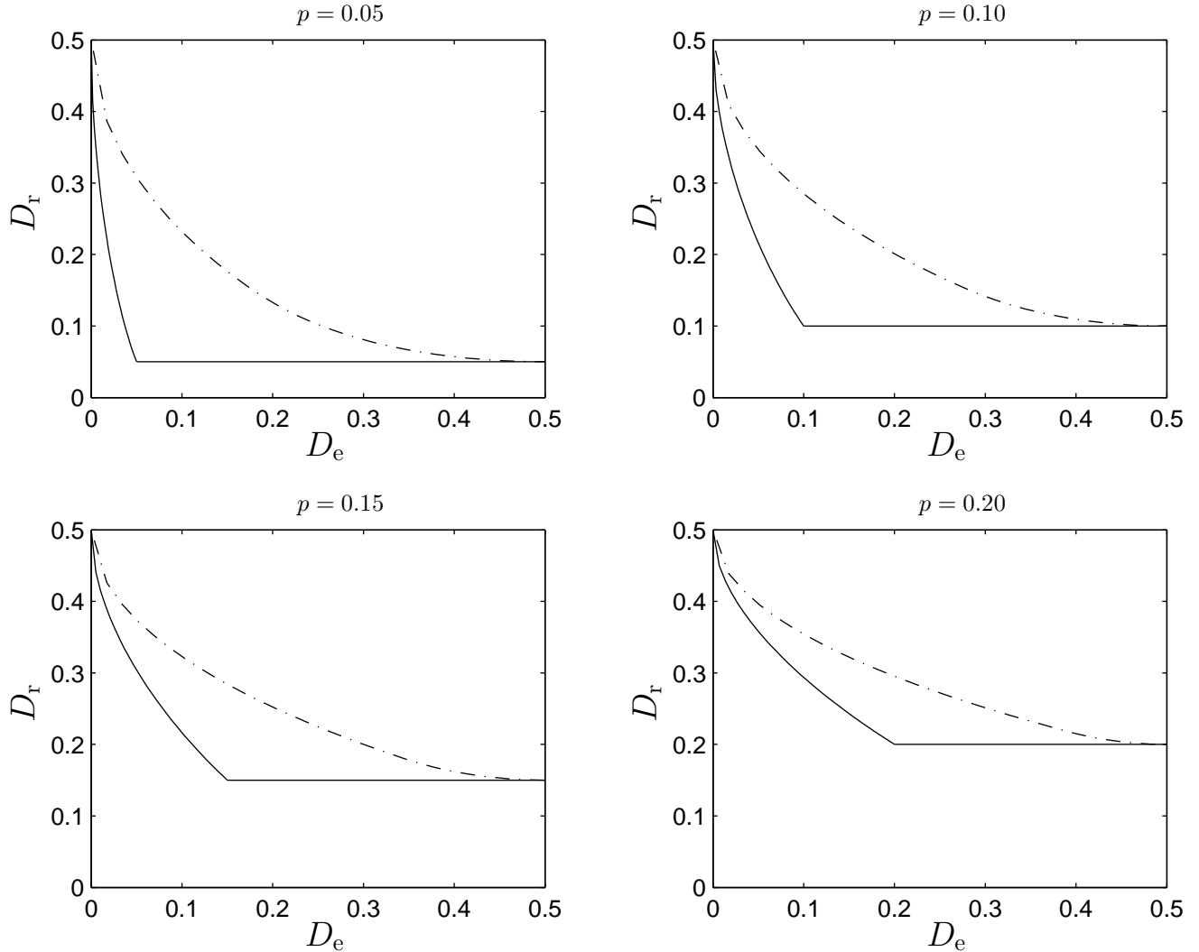
Fig. 6. Performance loss of quantize-and-embed systems for the Binary-Hamming scenario with various reference channel crossover probabilities p . The solid curve depicts the boundary of the achievable regions for the optimum system; the dashed curve depicts that of the best quantize-and-embed system.
