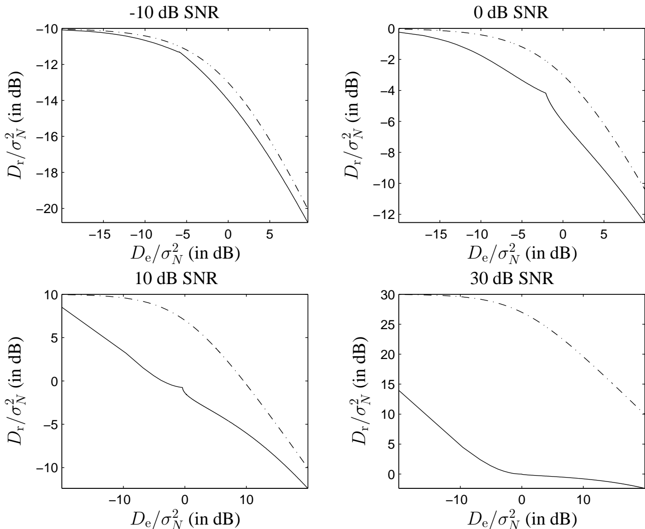
Fig. 7. Performance loss of quantize-and-embed systems for the Gaussian-quadratic scenario at various reference channel SNRs. The solid curve depicts the asymptotic outer bound of the achievable regions for the optimum system; the dashed curve depicts that of the best quantize-and-embed system.
