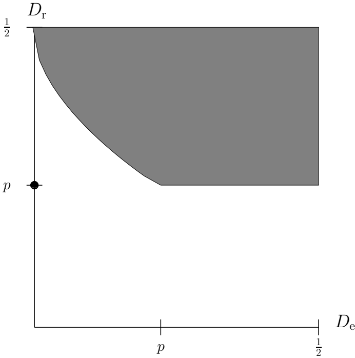
Fig. 2. The shaded area depicts the achievable distortion region for a symmetric Bernoulli source used in conjunction with a binary symmetric reference channel of crossover probability p . Distortions are with respect to the Hamming measure. The case p = 0 corresponds to traditional digital signatures. If authentication was not required, the point (D_e = 0, D_r = p) could be achieved.
