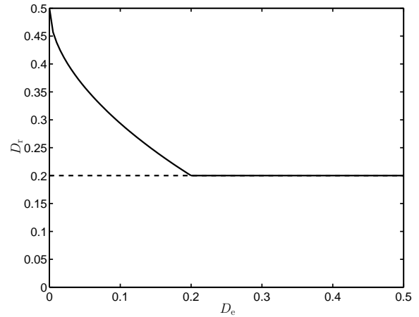
Fig. 4. The solid curve represents the frontier of the achievable distortion region for a binary symmetric source and a binary symmetric reference channel with cross-over probability p = 0.2 . This plot reflects the system behavior when the reference channel is in effect. The dashed line represents the boundary of the larger distortion region achievable when authentication is not required.
