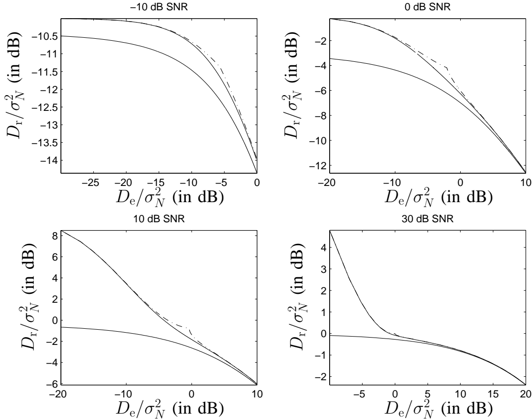
Fig. 5. Bounds on the achievable distortion region for the Gaussian-quadratic problem. The lowest solid curve is the inner bound corresponding to the boundary of the achievable region when reconstructions need not be authentic. The numerically obtained upper solid curve is the outer bound resulting from the use of Gaussian codebooks. The dashed curve corresponds to the lower convex envelope of the simple low and high D_e analytic outer bounds derived in the text.
