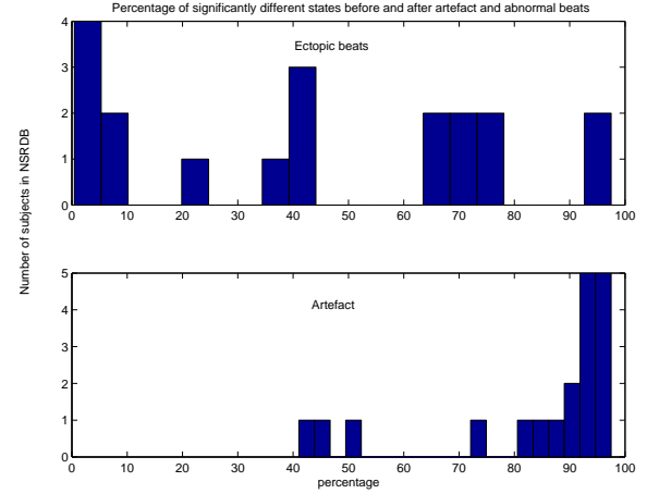
Figure 4. Percentage of significantly different states ( \mu_1 \neq \mu_2 or \sigma_1^2 \neq \sigma_2^2 ) in 100 second segments before and after artefact (lower plot) and ectopic beats (upper plot), tested using t- and F-tests for all 19 subjects in the Physionet NSRDB.
