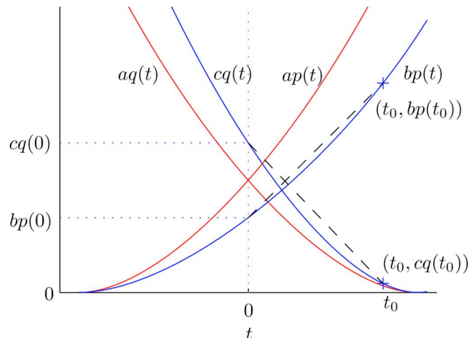
Fig. 2. Typical plot of the rate functions.
