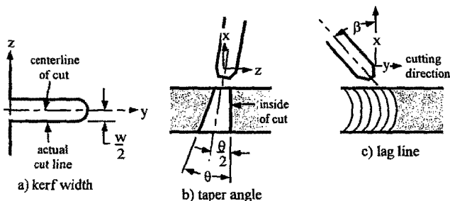
Fig. 10 Compensation methods for AWJ cutting error
