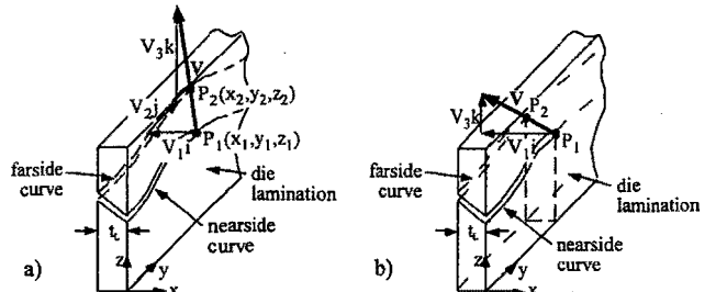
Fig. 5 Die lamination with an (a) compound bevel and (b) simple planar bevel
