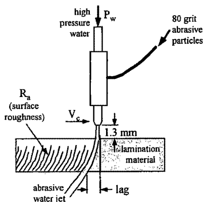
Fig. 9 Abrasive water jet cutting
