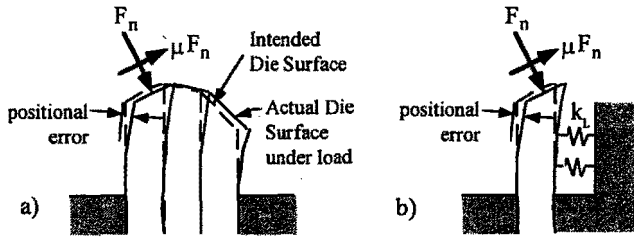
Fig. 2 (a) Group of die laminations subjected to generic forming loads and (b) modeled as cantilevered Euler beams in a parallel configuration
