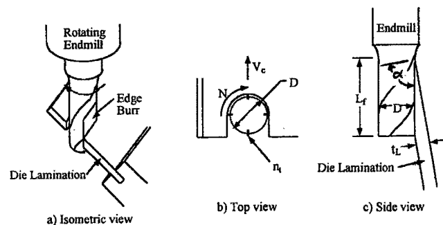
Fig. 8 Machining a lamination bevel with the flute-edge of an endmill
