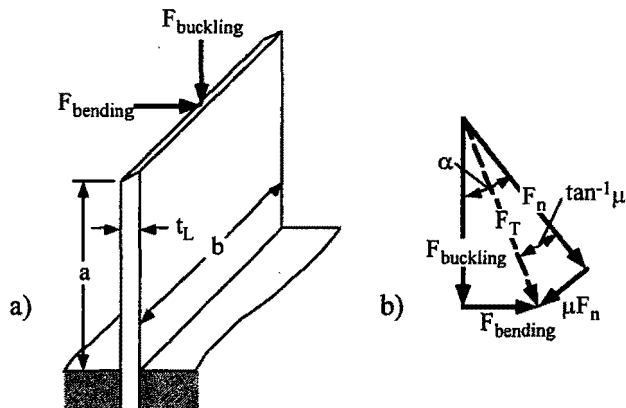
Fig. 3 (a) Single rectangular die lamination subjected to bending and buckling loads and (b) a vector diagram of all forming loads
