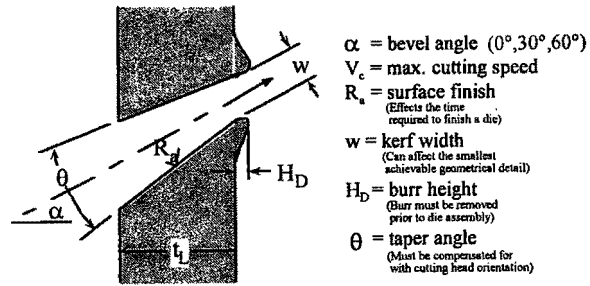
Fig. 7 Quality characteristics of a bevel cut
