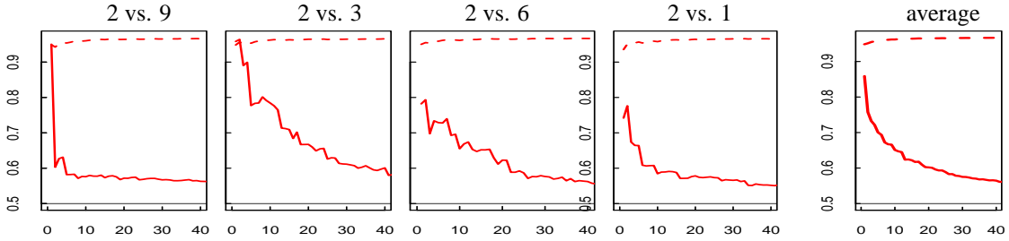
Figure 1: Area under ROC (AUROC) (y-axis) for predicting digit ‘2’ using the greedy algorithm. The x-axis shows the order of variables were picked out of 2000 total variables. The top dashed line shows generalization or ‘test’ performance on the source domain. The transfer to a new domain is shown below it as the solid line. The last figure on the right shows the average of all the ROC curves. The horizontal line is at “chance.”
