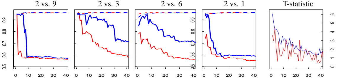
Figure 2: Area under ROC (AUROC) (y-axis) for predicting digit '2' for both the greedy algorithm (shown in red) and for our T -greedy algorithm (shown in blue), as we add more features (x-axis). Since we choose features based on T-statistics (see last graph), our T-statistics is generally higher than that of the greedy algorithm.
