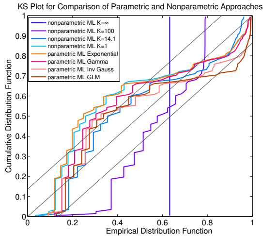
Fig. 1. Using the time-rescaling theorem and Kolmogorov-Smirnov plots for model selection of the Lipschitz parameter K . The optimization algorithm was applied to 3000ms of goldfish retinal ganglionic neural data and plotted are the 95% confidence intervals as well as empirical CDFs of the time-rescaled ISIs for K = 1.0 , K = 14.1 , and K = 100 .
