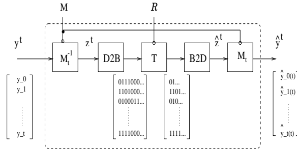
Fig. 2. Quantizer-Channel-Decoder Operator at Time t
