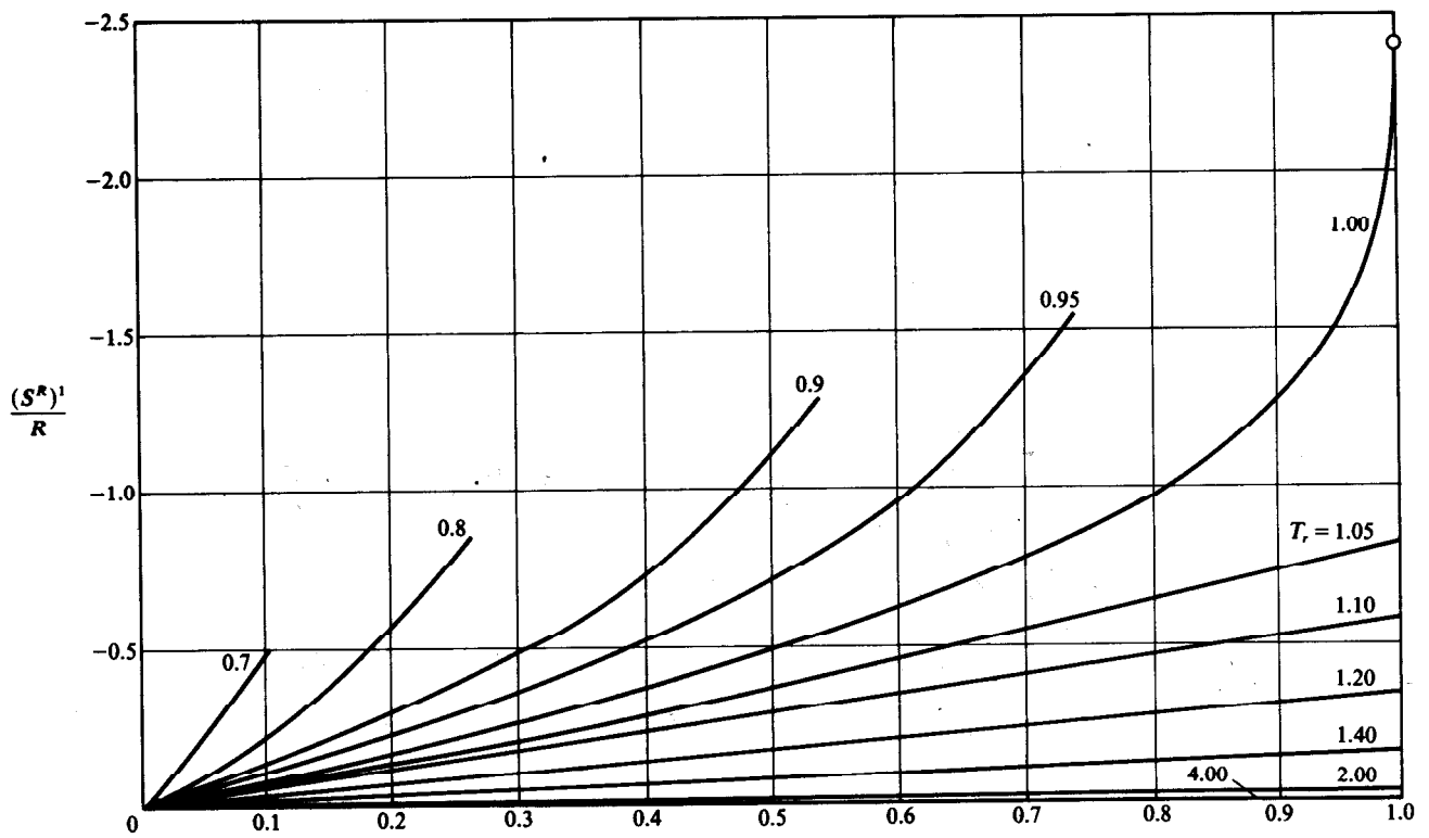
Figure 6.12 Generalized correlation for (S^R)^1/R , Pr < 1.0 . (Based on data of B. I. Lee and M. G. Kesler, ibid. )
