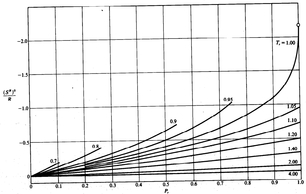
Figure 6.10 Generalized correlation for (S^R)^0/R, Pr < 1.0 . (Based on data of B. I. Lee and M. G. Kesler, ibid. )
