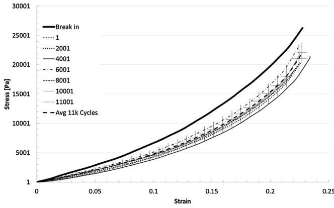
Fig. 4. Coarse steel wool sample loading behavior with initial thickness 8.5 mm and cyclically compressed to thickness 6.5 mm, and loaded at 2 mm/sec at a cycle frequency of 0.5 Hz. For clarity the data shown is for the loading portion of the test. The average is calculated taking the first sample of every thousand data set. The cross bars on the average line represent a standard deviation.
