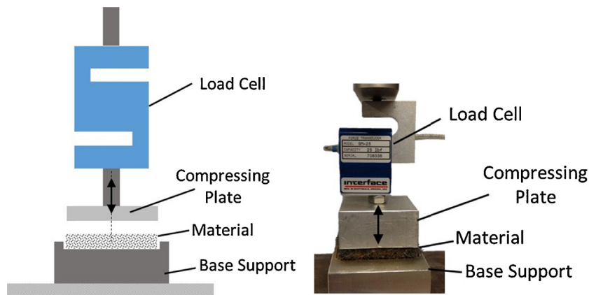
Fig. 1. System used to measure the cyclic stress–strain relation of the samples.
