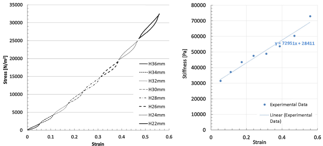
Fig. 6. (L) Stacked cycling response for densification sample. (R) Stiffness measured for the array of strain densification tests.
