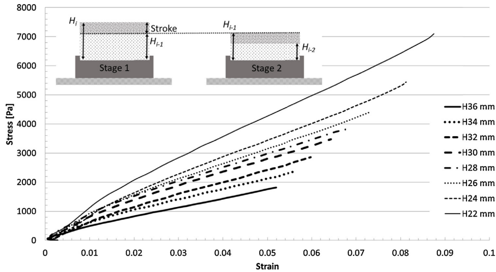
Fig. 5. Densification structure stress–strain curve of the loading section at each height.
