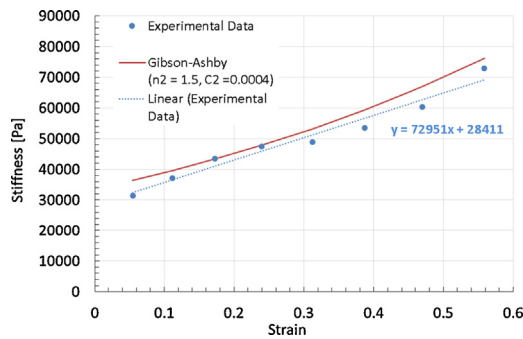
Fig. 9. Strain versus stiffness behavior for the densification experiment with an overlay of the Gibson–Ashby model.
