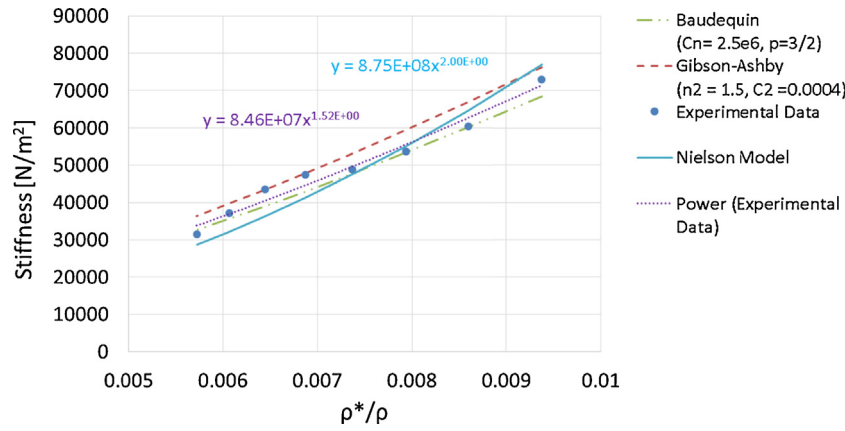
Fig. 7. Analytical model comparison between experimental data and analytical model.
