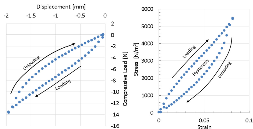
Fig. 3. Typical loading and unloading data from the tester and engineering stress–strain representation for the coarse sample.
