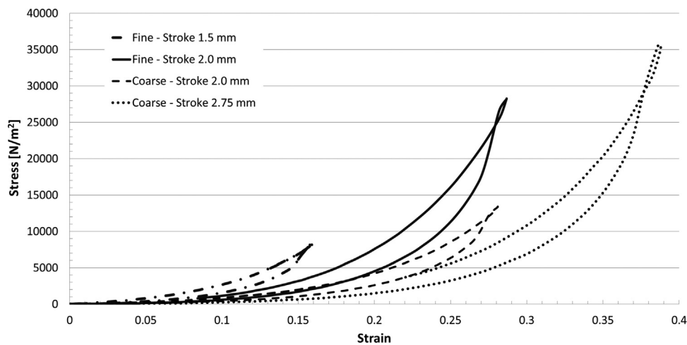
Fig. 2. Coarse versus fine characterization. Height of fine sample is 13.7 mm and coarse sample 14.0 mm. The data shown is for a complete cycle of load/unload. The stroke refers to the compression of the sample.
