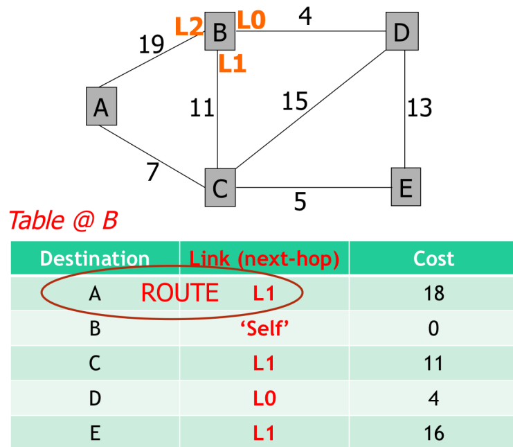
Figure 18-2: A simple network topology showing the routing table at node B. The route for a destination is marked with an oval. The three links at node B are L0, L1, and L2; these names aren't visible at the other nodes but are internal to node B.
