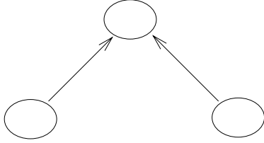
Figure 2: A single cell configuration where all stations are in range of each other and both pads are sending data to the base station (the arrows indicate the direction of the data transmission). The pads are each generating data at a rate of 64 packets per second and are using UDP for transport.
