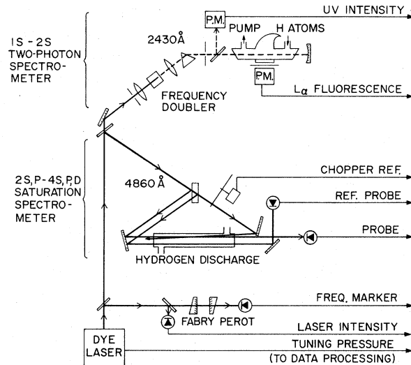
FIG. 1. Experimental setup.
