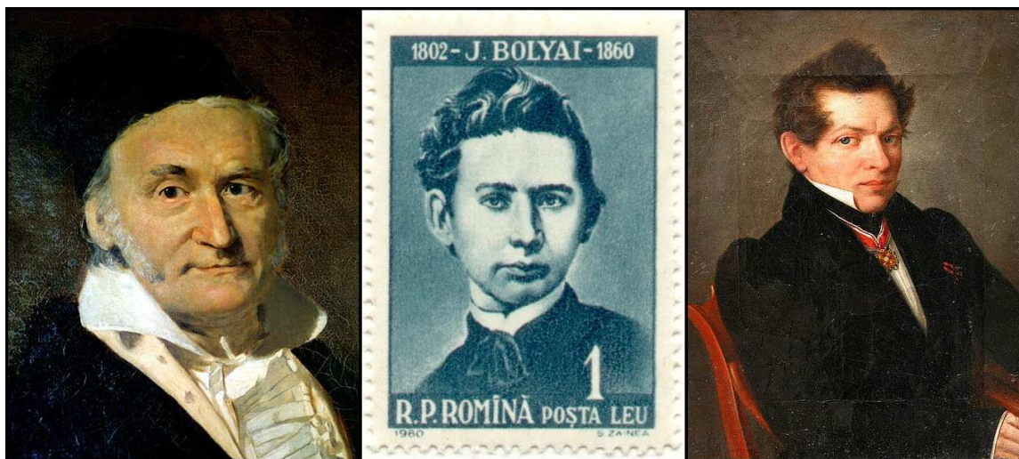
Figure 5.4: Carl Friedrich Gauss, János Bolyai, and Nikolai Ivanovich Lobachevsky independently developed the first example of a mathematical theory in which Euclid's fifth postulate is false, now known as the Gauss–Bolyai–Lobachevsky geometry. Gauss (1777–1855) was the son of poor working-class parents in Germany, but by the time he was 15 his mathematical talents were noticed by the Duke of Brunswick, who sent Gauss to the Collegium Carolinum and then the University of Göttingen. Gauss remained at Göttingen for the rest of his life, becoming Professor of Astronomy and director of the astronomical observatory in 1807. His students included Richard Dedekind, Bernhard Riemann, Peter Gustav Lejeune Dirichlet, Gustav Kirchhoff, August Ferdinand Möbius, and Friedrich Bessel. Bolyai (1802–1860) was the son of Farkas Bolyai, a teacher of mathematics, physics, and chemistry at the Calvinist College in Marosvásárhely, Hungary (now Tirgu-Mures, Romania). Although his father was well-educated, he was nonetheless not well paid, so János attended Marosvásárhely College and later studied military engineering at the Academy of Engineering at Vienna, because that is what they could afford. He then entered the army engineering corps, where he served for 11 years, during which time he carried out his now-famous investigation of non-Euclidean geometry. The work was published in 1831 as an appendix in a book written by his father. Bolyai resigned from the army in 1833 due mainly to health problems, and lived the rest of his life in relative poverty, dying at the age of 57 of pneumonia. The Romanian postage stamp shown here honored the 100th anniversary of Bolyai's death; the picture was apparently fabricated, as no authentic picture of Bolyai is known to exist. Lobachevsky (1792–1856) was the son of Polish parents living in Russia. His father was a clerk in a land-surveying office, who died when Lobachevsky was only seven. His mother relocated the family to Kazan, Russia, where Lobachevsky attended Kazan Gymnasium and later was given a scholarship to Kazan University, where one of his professors was Martin Bartels, who was a teacher and friend of Gauss. Lobachevsky remained at Kazan University for the rest of career, becoming rector of the university in 1827. His work on non-Euclidean geometry was published in the Kazan Messenger in 1829, but was rejected for publication by the St. Petersburg Academy of Sciences. Lobachevsky was asked to retire in 1846, and after that his health and financial situation deteriorated, he became blind, and his favorite eldest son died. Lobachevsky himself died before the importance of his work in mathematics was appreciated.
