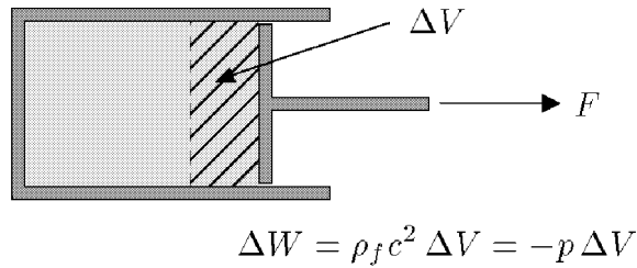
Figure 10.3: The piston of the thought experiment is pulled out, enlarging the chamber. The energy density of the false vacuum inside the chamber is fixed, so the energy in the chamber goes up. The energy must come from the agent that pulled on the piston. For the agent to do positive work, the pressure inside the chamber must be negative.
