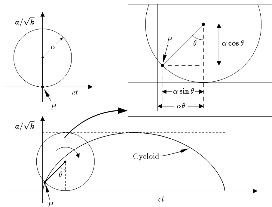
Figure 4.1: Evolution of a closed universe. The figure shows a graph of a/\sqrt{k} vs. ct for a closed matter-dominated universe. If one imagines a circle rolling on the ct axis, a point on the circle traces out a cycloid, which is exactly the equation for a/\sqrt{k} for a closed universe. The insert at the upper right includes labels for various distances, showing the connection with Eq. (4.25).
