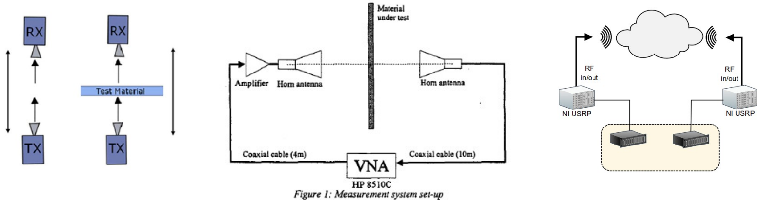
Figure 1: Measurement system set-up
