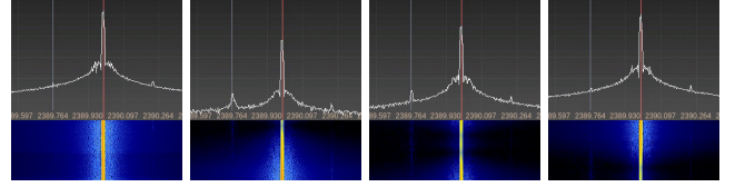
Figure 3: The real-time FFT readings shown as a metallic lunchbox with a concealed peanut butter container is scanned (see Figure 4). A decrease is visible in the spectrogram as well as in the FFT while the antennas move through the region with the object.
