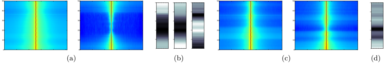
Figure 2: (a) Spectrograms at each trajectory segment for a horizontal scan of free-space and a metallic box at 2390 MHz (see Figure 4). (b) Losses at each segment when scanning the metallic box and the metallic box with a concealed object along with the resulting difference. (c) Spectrograms at each trajectory segment for a horizontal scan of a plastic box and a plastic box with a concealed object (see Figure 7). (d) The resulting difference in loss at each segment for the measurements shown in (c).
