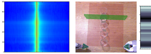
Figure 5: Horizontal scan of several plastic cups (one with water) at 4.39 GHz. The spectrograms measured at each location are shown on the left. A estimated size and location of the cup containing water is shown as a green rectangle in the range-image. The loss sequence used for the estimate is shown besides the range-image. This sequence is the result of the difference in loss between a free-space scan and the scan of the cups.
