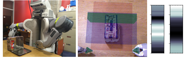
Figure 4: Horizontal scan of a metallic box with a concealed peanut butter container at 2.39 GHz. The estimated location and size of the box and object are displayed in the range-image as the blue and green rectangles respectively. The loss sequences used for the estimates are shown besides the range-image.
