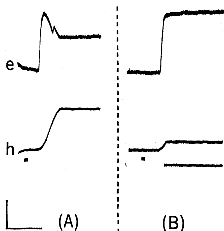
Fig. 3. (A) Typical coordinated eye ( e ) and head ( h ) response to sudden appearance of a target. (B) Presentation of the same target is followed by application of the brake (horizontal bar). Note lack of compensatory eye movement. Dots represent onset of luminous target. Calibration: horizontal bar equals 500 msec; vertical bar, 15 degrees.
