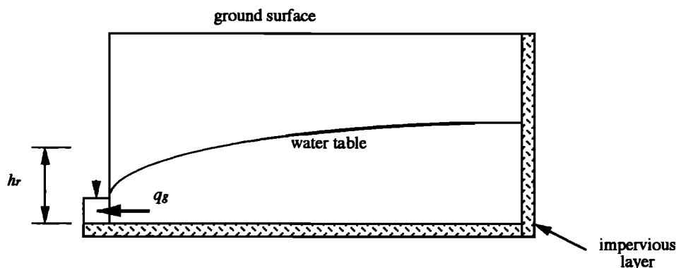
Figure 16. A schematic figure describing the simple groundwater flow configuration that has been assumed in developing equation (9).
