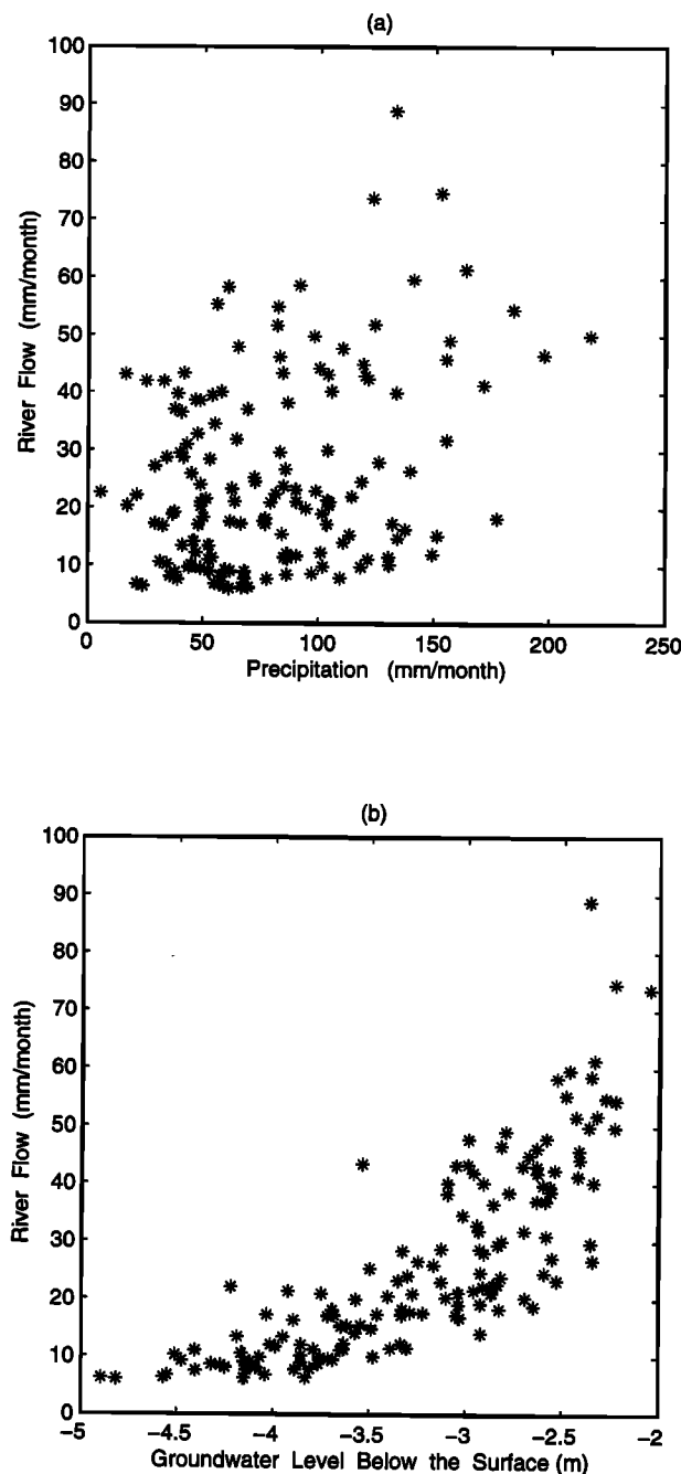
Figure 12. Plots of monthly (a) precipitation and (b) groundwater level versus monthly river flow during 1983–1994 in Illinois.
