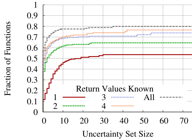
Figure 3-5: textttlibc function CDF as return values are learned.
