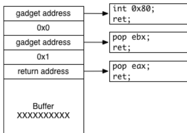
Figure 2-1: basic ROP that calls exit()
