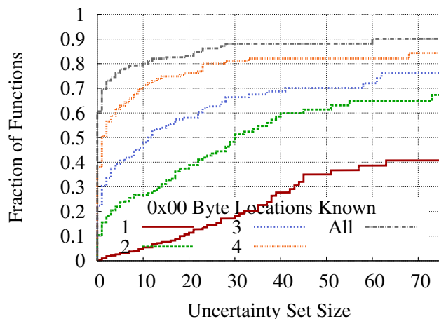
Figure 3-2: Uncertainty set size of textttlibc functions upon leaking null byte locations.
