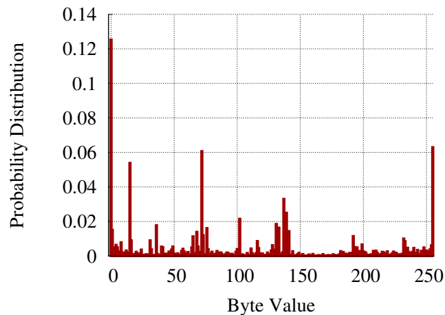
Figure 3-1: Byte value distribution in textttlibc .
