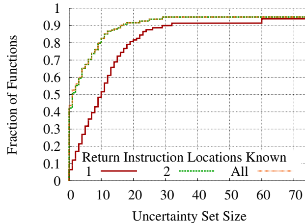
Figure 3-3: Uncertainty set size of textttlibc functions depending on number of leaked return instructions.
