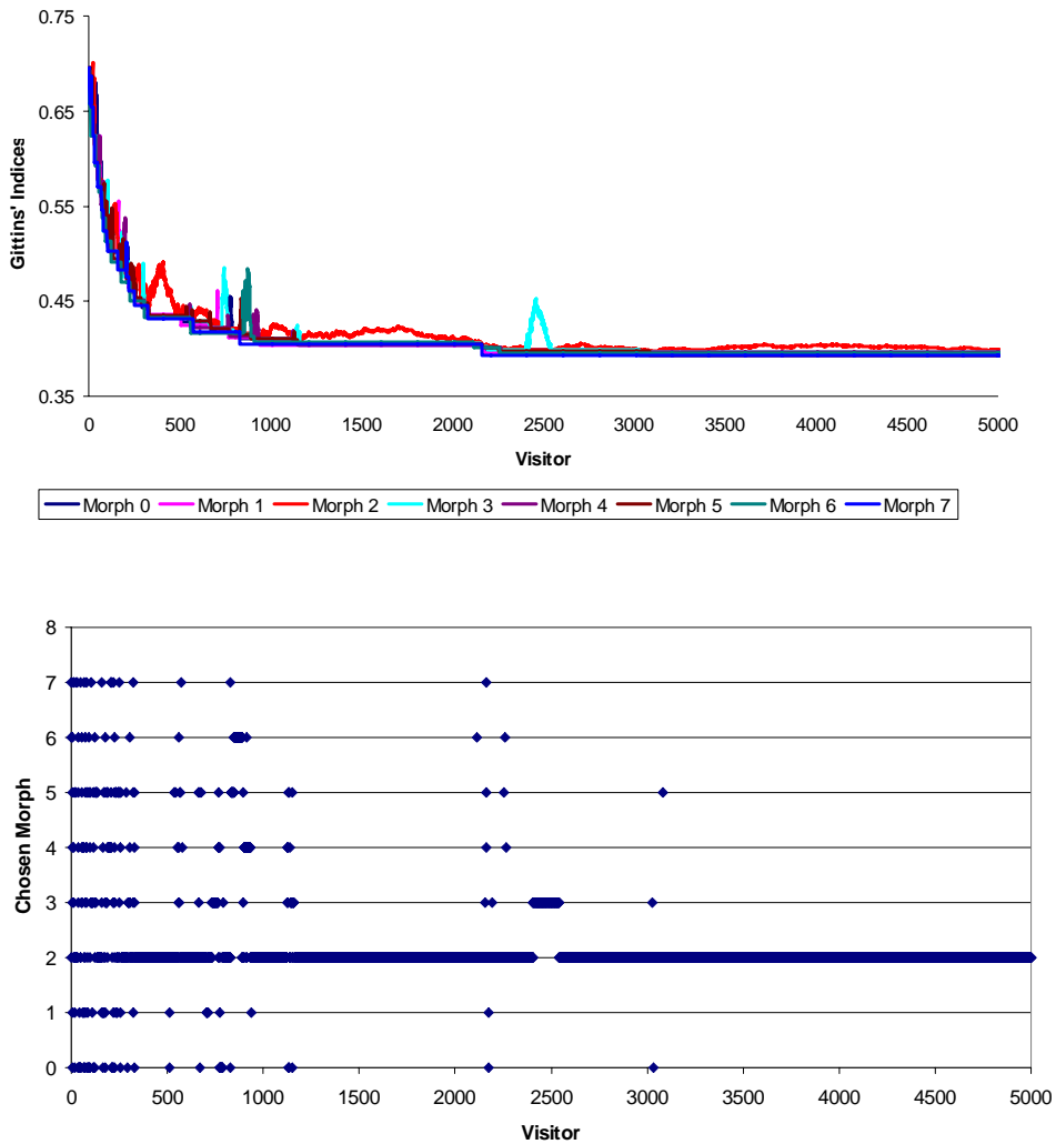
Figure 3 Evolution of the Dynamic Programming Loop
