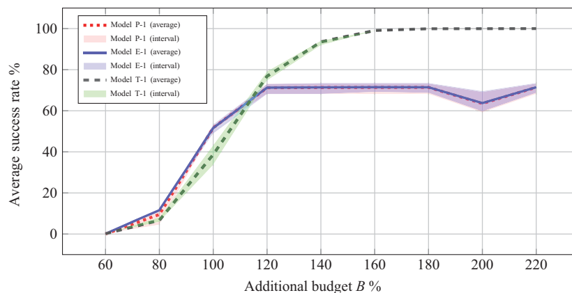
Figure 1. (Color online) Success Rates for Models T-1, P-1, and E-1
