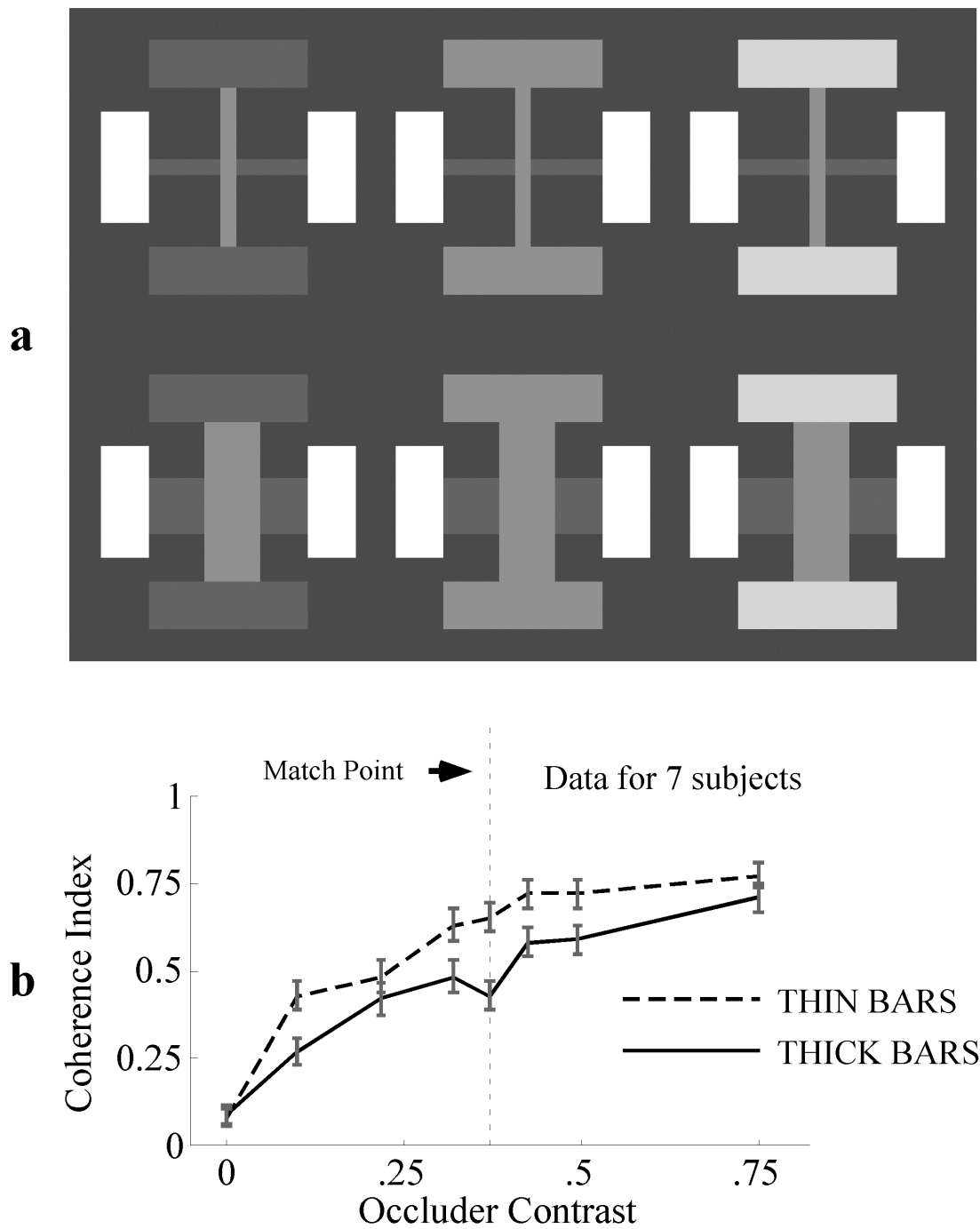
Figure 9. To control for resolution issues, we repeated the first experiment with bars that were 3.5 times as thick. Changing the junctions at the bar endpoints again has little to no effect.
