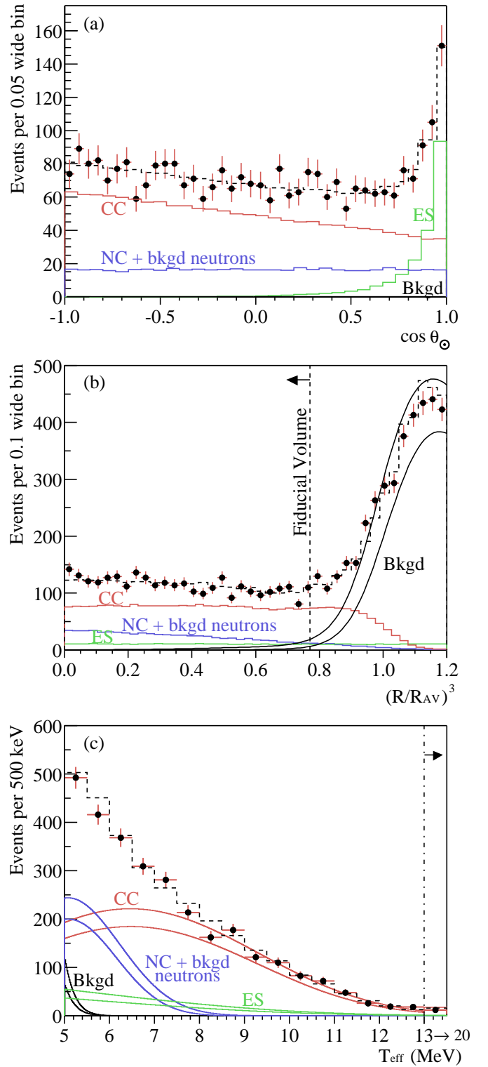
FIG. 2: (a) Distribution of \cos \theta_{\odot} for R \leq 550 cm. (b) Distribution of the volume weighted radial variable (R/R_{\text{AV}})^3 . (c) Kinetic energy for R \leq 550 cm. Also shown are the Monte Carlo predictions for CC, ES and NC + bkgd neutron events scaled to the fit results, and the calculated spectrum of Cherenkov background (Bkgd) events. The dashed lines represent the summed components, and the bands show \pm 1\sigma uncertainties. All distributions are for events with T_{\text{eff}} \geq 5 MeV.
