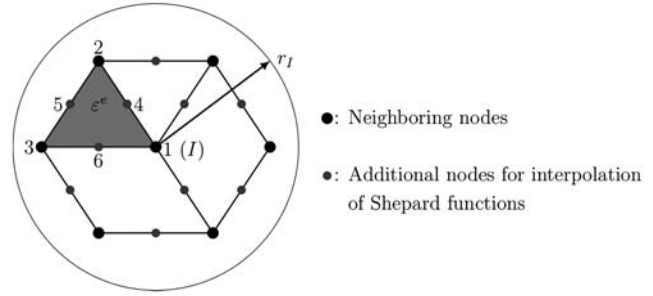
Fig. A.1. Interpolation of the Shepard functions on a triangular overlapped region \epsilon^\epsilon .
