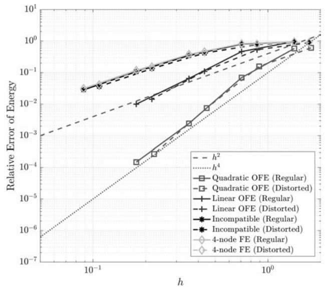
Fig. 9. The ad-hoc problem: convergence rates; h is the mean element size (diameter of smallest circle encompassing the element) [1].
