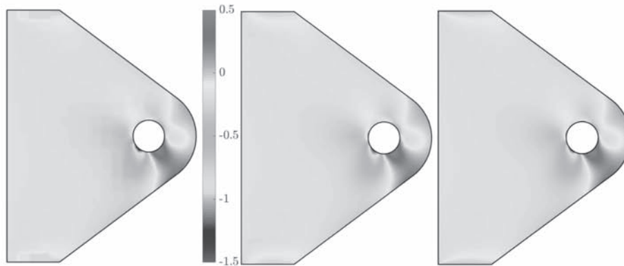
b) Left AMORE mesh ( \sigma_{sy\max} = 0.4728, \sigma_{sy\min} = -1.4525 ) Middle: Traditional mesh ( \sigma_{sy\max} = 0.4625, \sigma_{sy\min} = -1.3187 ) Right Reference solution ( \sigma_{sy\max} = 0.4680, \sigma_{sy\min} = -1.4604 )
