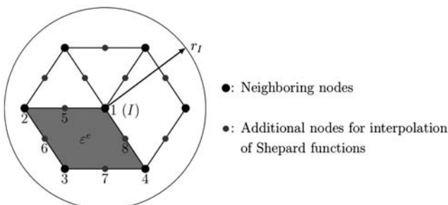
Fig. 3. Nodal positions (nodes 1, 2, 3, 4) of the Shepard functions and nodes used for the interpolation of the Shepard functions (nodes 1–8) for the quadrilateral 4-node element e^e .
