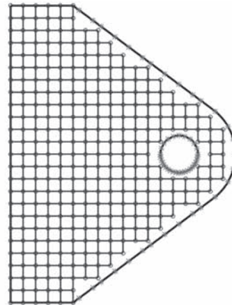
b) Step 2: The boundary is discretized; Cells outside or cutting the domain are removed
