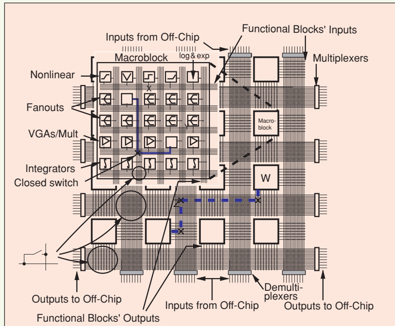
Block diagram of the analog-computer integrated circuit developed by Cowan, Melville, and Tsividis. The function blocks are divided into a 4 \times 4 array of macroblocks, as shown in the detail. Crosspoint switches route signals from the function blocks around the chip to other blocks, allowing the analog computer to be quickly programmed to solve differential equations. The figure shows the output of block X patched to the input of block Y and the output of macroblock W patched to the input of macroblock Z.
