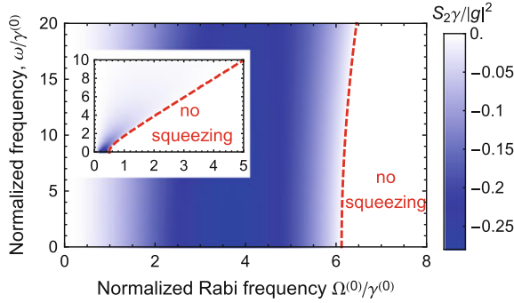
Fig. 2.4 a Squeezing spectrum of the out-of-phase quadrature ( S_2 ) as a function of \omega/\gamma^{(0)} and \Omega^{(0)}/\gamma^{(0)} , respectively. The spectrum is normalized by |g|^2/\gamma . Same geometrical parameters as in Fig. 2.3. The pure dephasing rate \gamma^* is neglected. Inset: analogous representation in the absence of GNS. Adapted from [14]. © IOP Publishing. Reproduced with permission. All rights reserved
