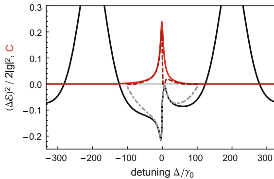
Fig. 2.8 Electric field fluctuations (black curve) optimized by the detection quadrature angle and steady state concurrence (red curve) versus laser detuning at \Omega^{(0)} = 60\gamma^{(0)} . Parameters as in Fig. 2.7. Negative values indicate squeezed light. The dash-dotted and dashed lines correspond to the two-level approximation on the |E\rangle - |G\rangle -transition for squeezing, and concurrence, respectively. Reprinted with permission from [16]. Copyright 2015 American Chemical Society
