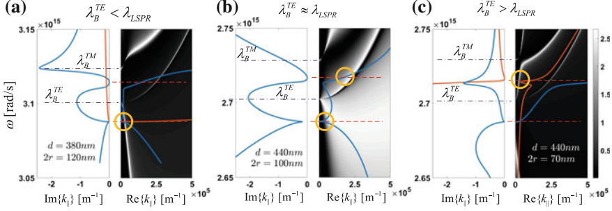
Fig. 8.8 Lasing versus detuning. a \lambda_B^{TE} < \lambda_{LSPR} . Left dispersion of imaginary part of k_{||} , distributed resonances takes place at the minimum points. Right dispersion of the real part of k_{||} . Greyscale image coupling between the excited mode to radiation. b as (a) but with \lambda_B^{TE} = \lambda_{LSPR} . c as (a) but with \lambda_B^{TE} > \lambda_{LSPR}
