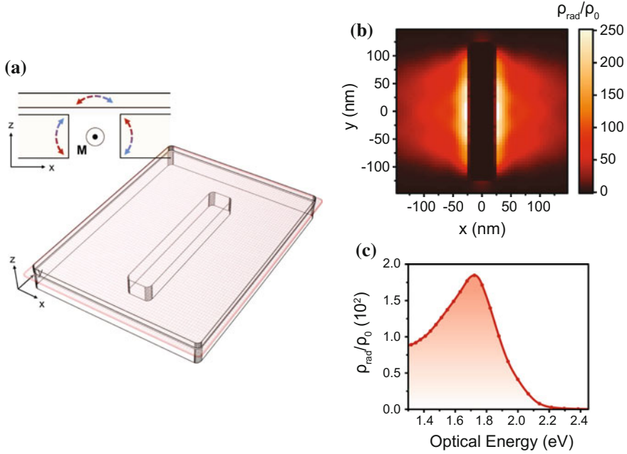
Fig. 10.8 a Sketch of an isolated slot antenna integrated in a MIM geometry. The plane indicates the region over which we evaluate the LDOS in the tunnel gap (c.f. panel (b) ). Electron to far-field radiation coupling is facilitated by a magnetic dipole mode along the long axis of the mode as indicated in the cross-section. Arrows represent the current distribution associated with this mode. b Normalized radiative LDOS \rho_{\text{rad}} = \rho_p \times \eta_{\text{antenna}} calculated as a function of position in the tunneling gap at an energy of 1.7 eV. The LDOS is maximal in the vicinity of the long axis of the 250 \times 50 \times 50 \text{ nm}^3 slot. c Radiative LDOS spectrum at a distance of 5 nm from the antenna edge
