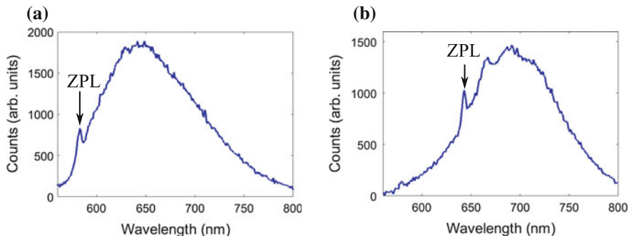
Fig. 3.8 Spectra of emission from a a single NV^0 and b a single NV^- center. Zero phonon lines (ZPL) are indicated with arrows
