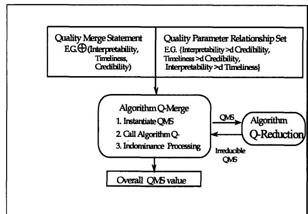
Figure 8: The Quality-Merge Statement (QMS)
