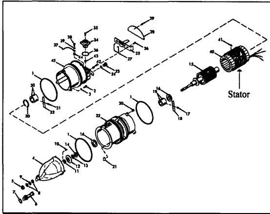
Figure 2: Stator position in the Fuel Booster Pump
