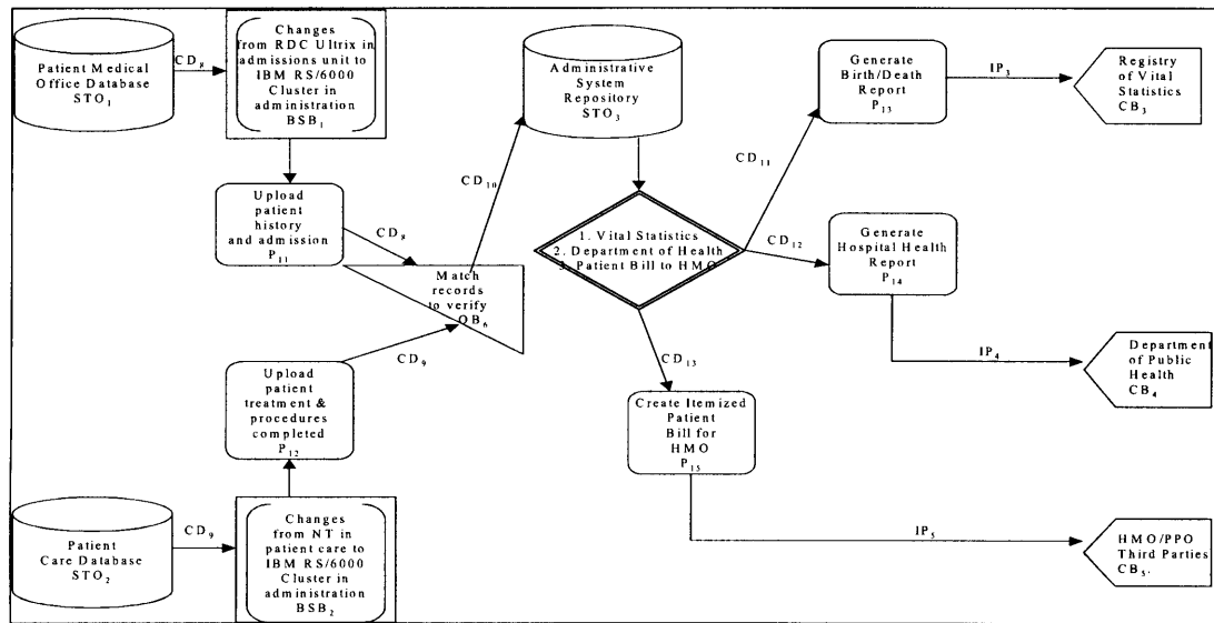
Figure 6: IPMap for Vital Statistics Report, Hospital Health Report, and Bill
